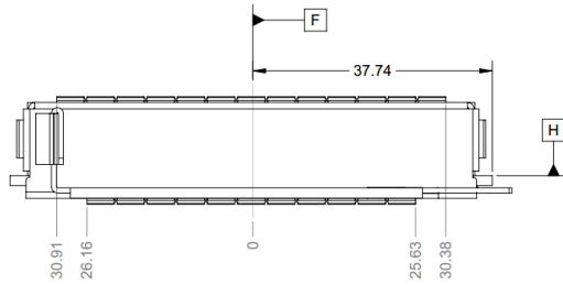
Figure 21: Small Form Factor OCP NIC 3.0 Card with Ejector CTF Dimensions (Side View)
