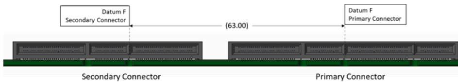
Figure 74: Primary and Secondary Connector Locations for Large Card Support with Right Angle Connectors
