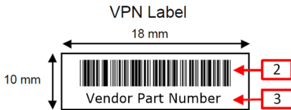
Figure 52: OCP NIC 3.0 Card Vendor Part Number Label
