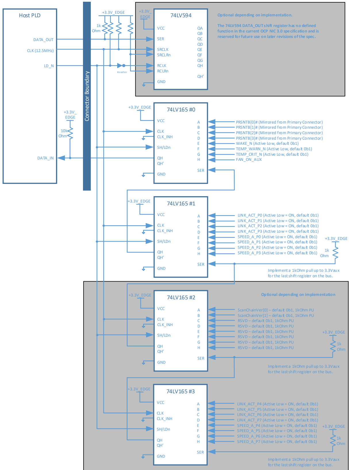
Figure 75: Scan Bus Connection Example
