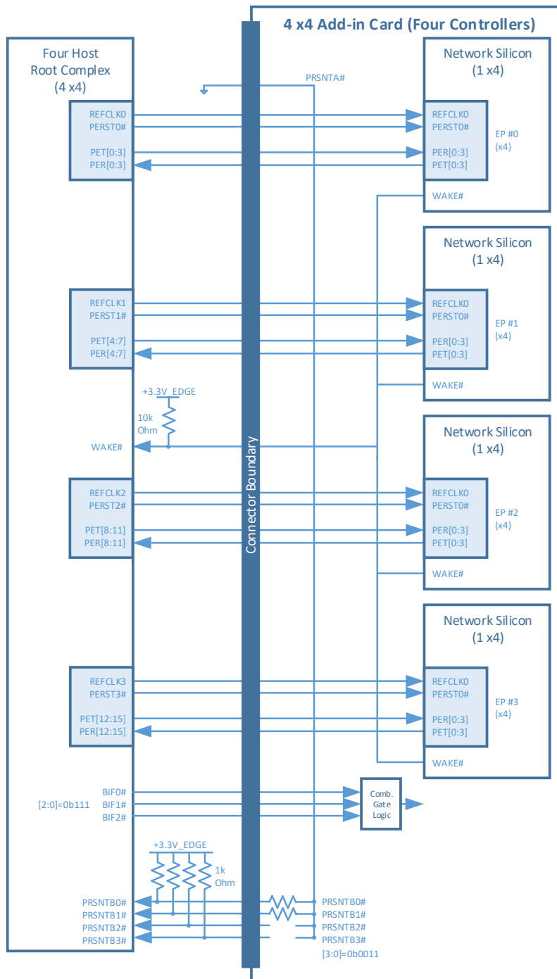
Figure 79: Quad Hosts (4 x4) and 4 x4 OCP NIC 3.0 Card (Quad Controllers)
