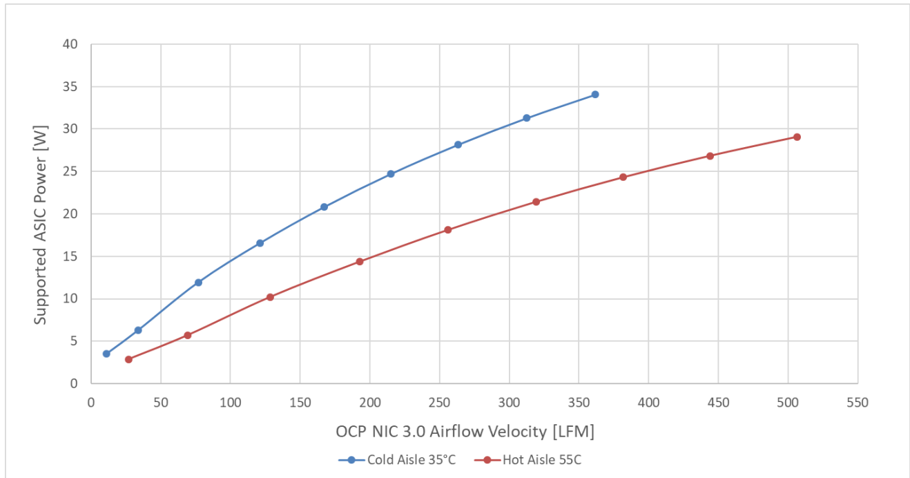
Figure 93: ASIC Supportable Power Comparison – Small Card Form Factor
