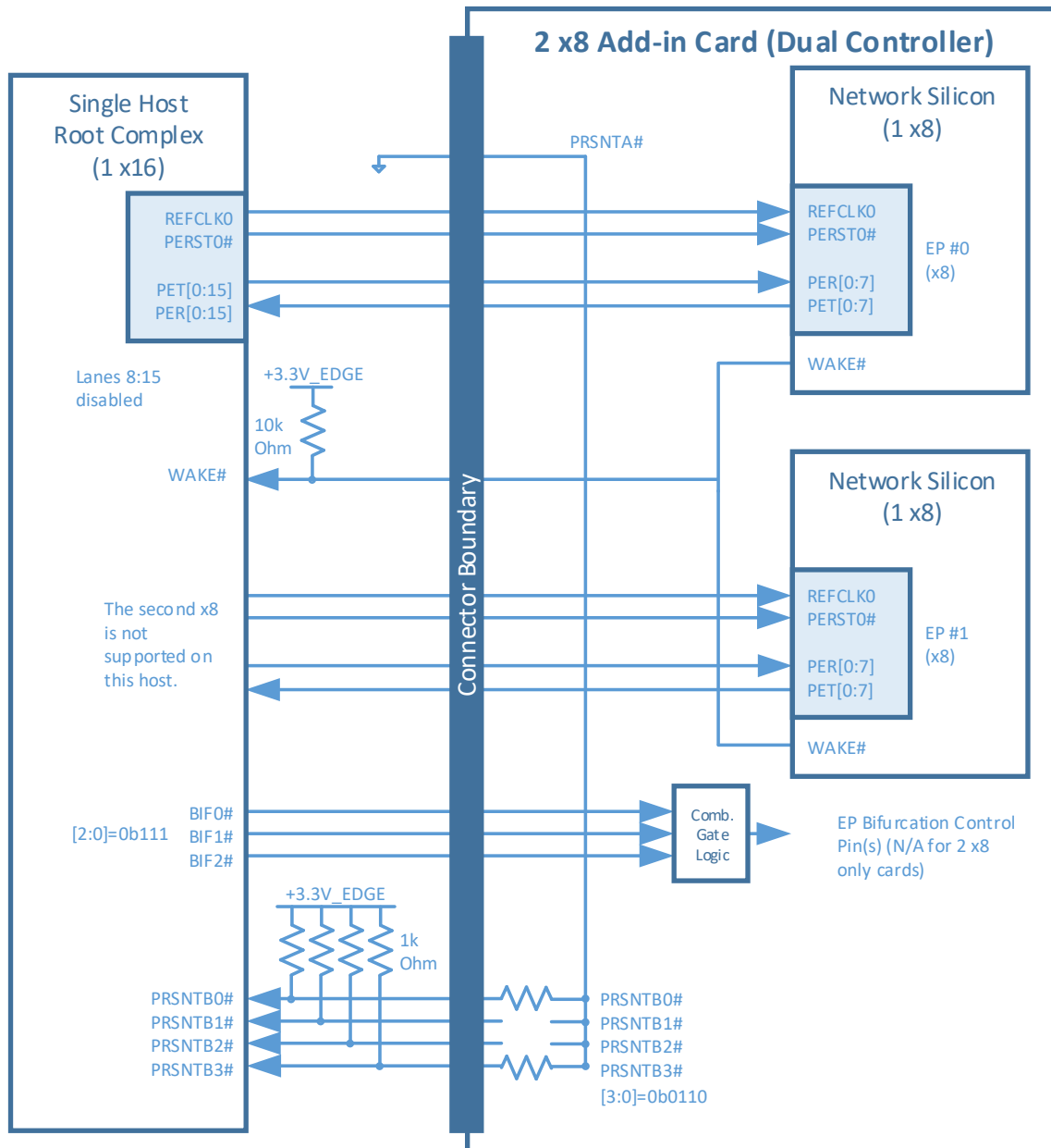
Figure 80: Single Host with no Bifurcation (1 x16) and 2 x8 OCP NIC 3.0 Card (Dual Controllers)
