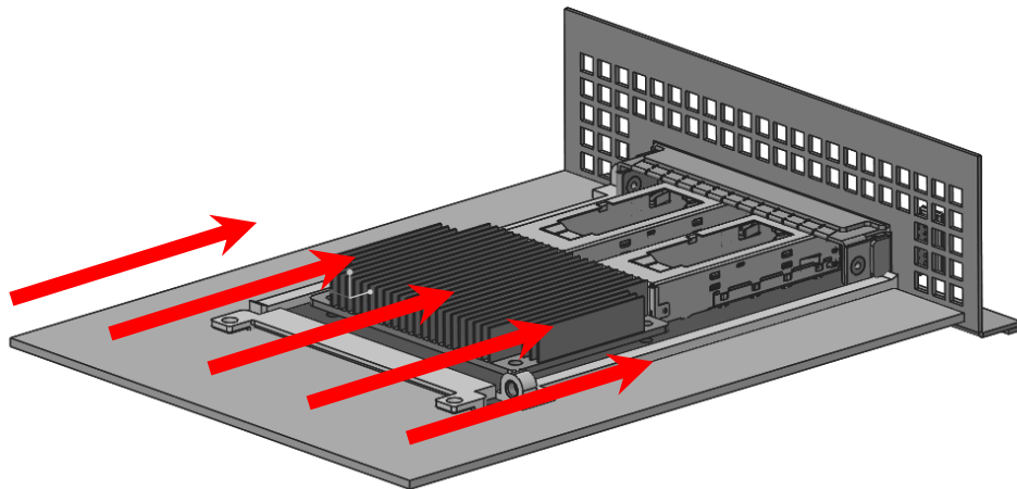
Figure 86: Airflow Direction for Hot Aisle Cooling
