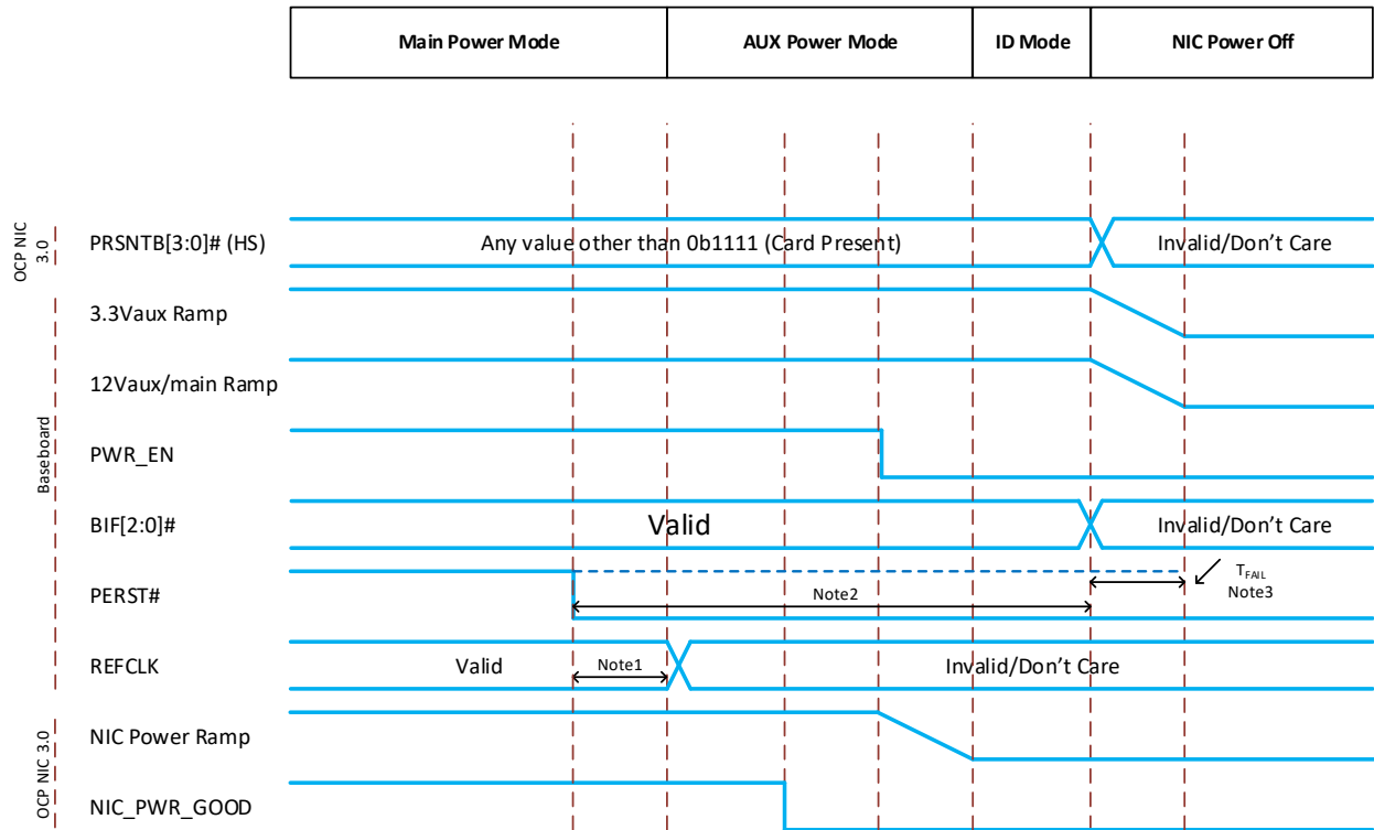
Figure 85: Power-Down Sequencing
