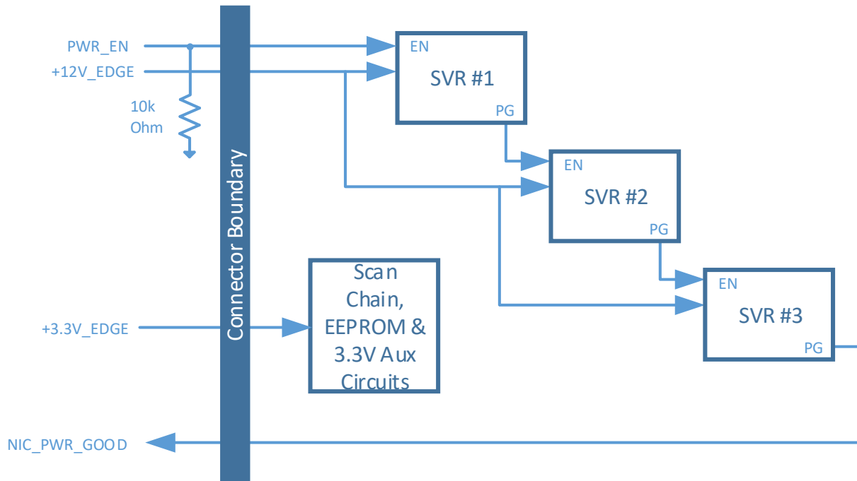
Figure 71: Example Power Supply Topology
