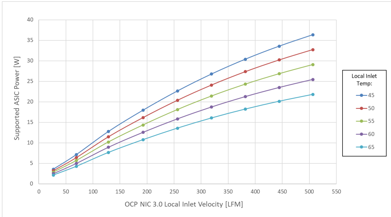
Figure 88: ASIC Supportable Power for Hot Aisle Cooling – Small Card Form Factor
