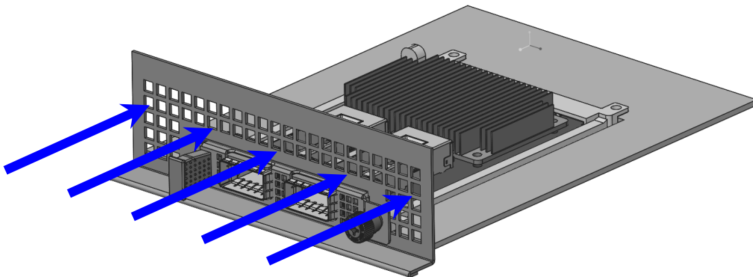
Figure 87: Airflow Direction for Cold Aisle Cooling
