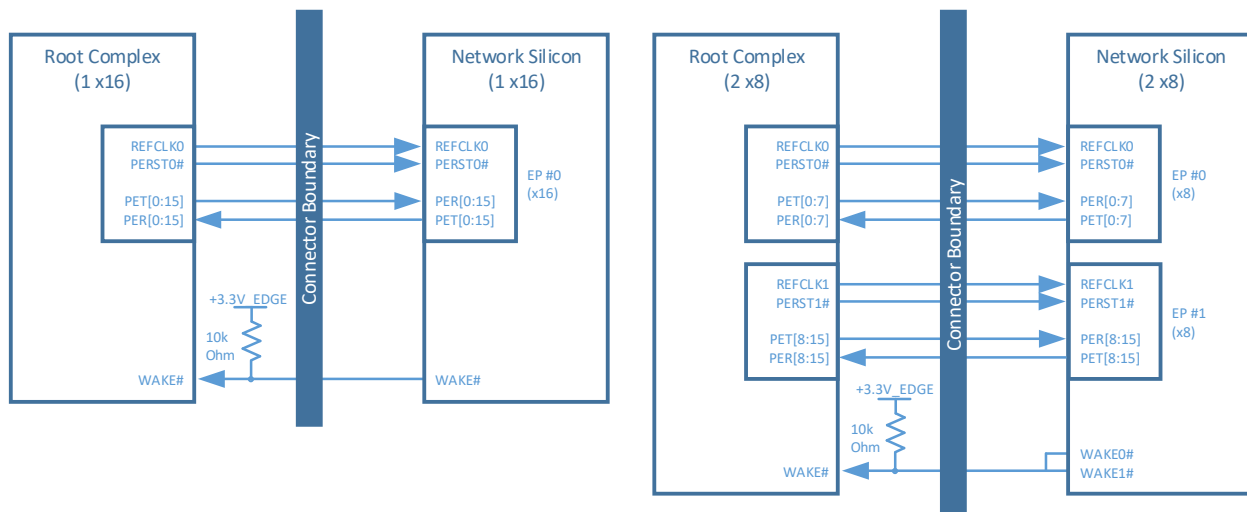
Figure 81: PCIe Interface Connections for 1 x16 and 2 x8 OCP NIC 3.0 Cards
