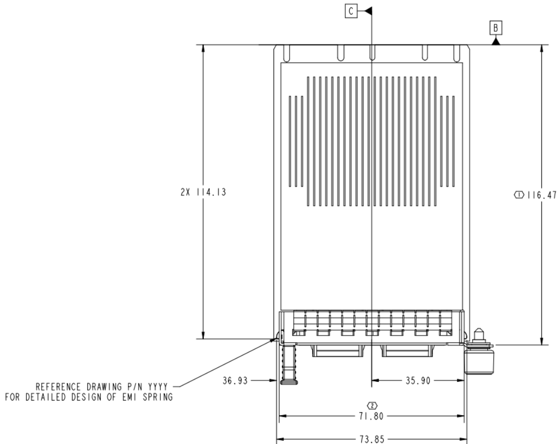
Figure 13: Small Form Factor OCP NIC 3.0 Card Critical-to-Function (CTF) Dimensions (Top View)
