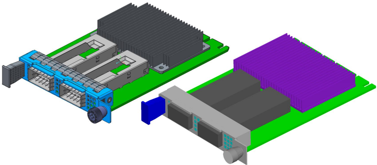
Figure 89: OCP NIC 3.0 Reference Geometry CAD & CFD
