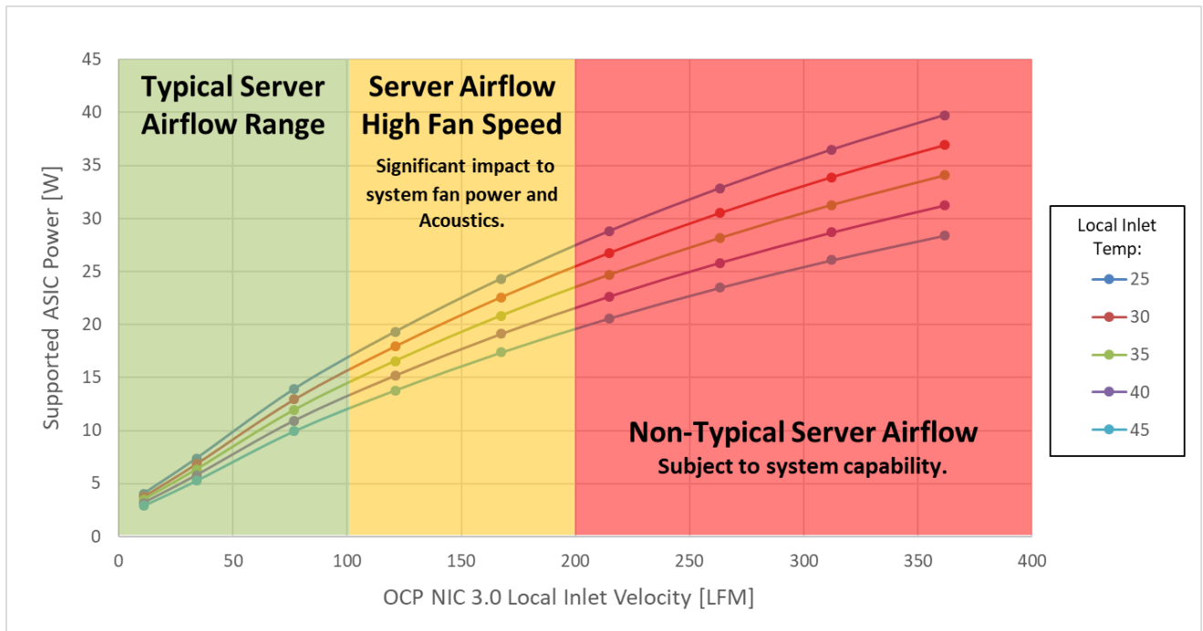
Figure 92: Server System Airflow Capability – Cold Aisle Cooling
