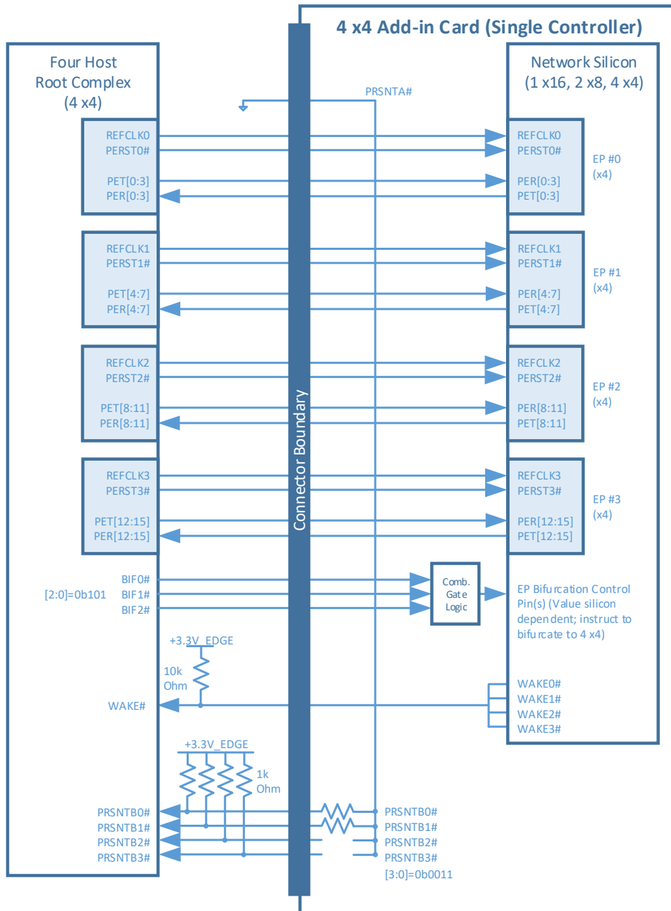
Figure 78: Quad Hosts (4 x4) and 4 x4 OCP NIC 3.0 Card (Single Controller)
