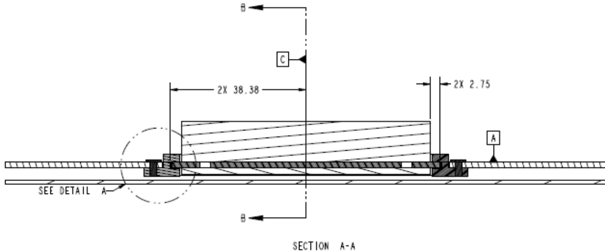
Figure 20: Small Form Factor Baseboard Chassis Critical-to-Function (CTF) Dimensions (Rail Guide Detail)
