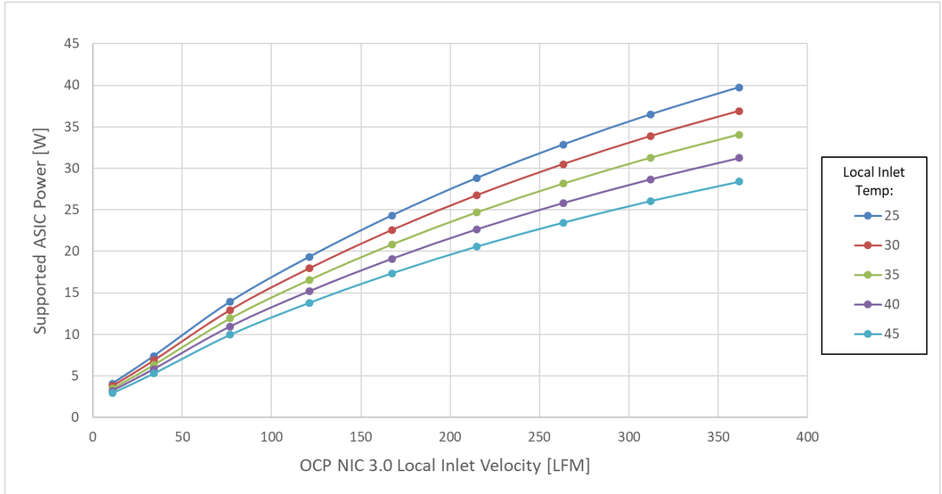
Figure 91: ASIC Supportable Power for Cold Aisle Cooling – Small Card Form Factor
