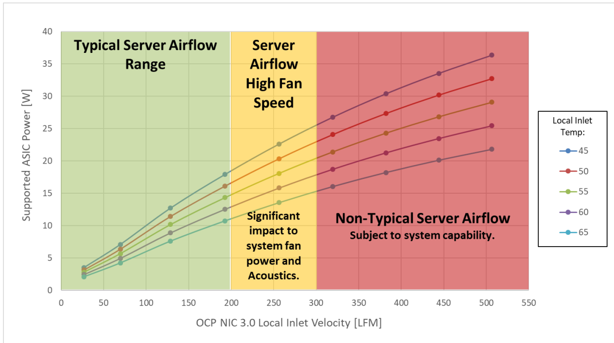
Figure 90: Server System Airflow Capability – Hot Aisle Cooling
