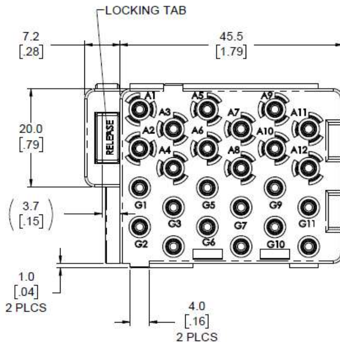
Figure 49 :Open19 Power Shelf Output Connectors Pinout (External View)
