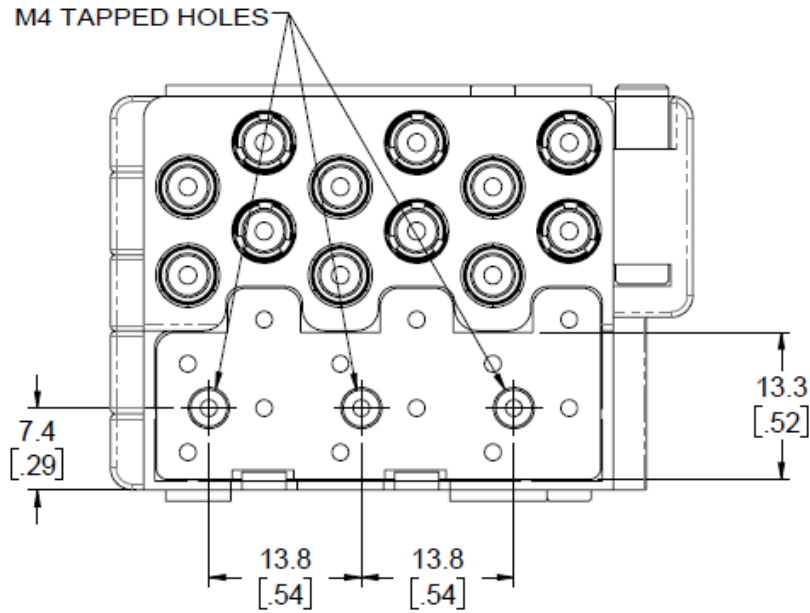
Figure 61 : Open19 Power Shelf Output Connectors Pinout (Internal View)
