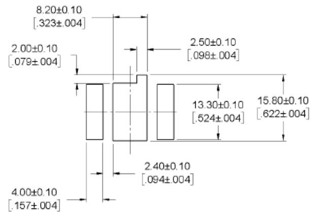
Figure 13 :12RU Power Cutout
