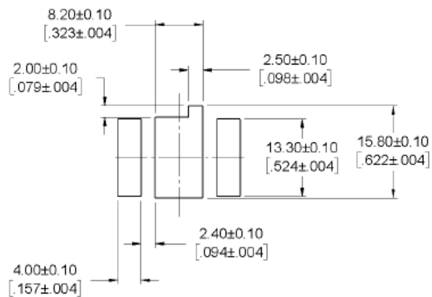
Figure 32 :8RU Power Connector Cutout
