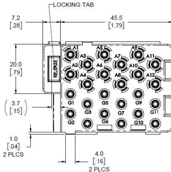
Figure 60 :Open19 Power Shelf Output Connectors Pinout (External View)
