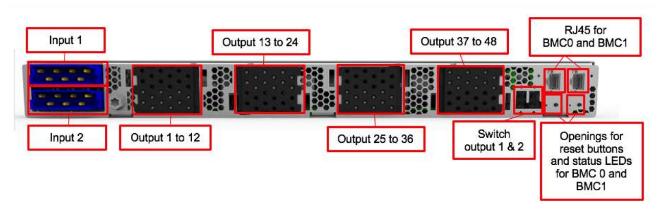
Figure 58 :Open19 Power Shelf Rear Connectors View
