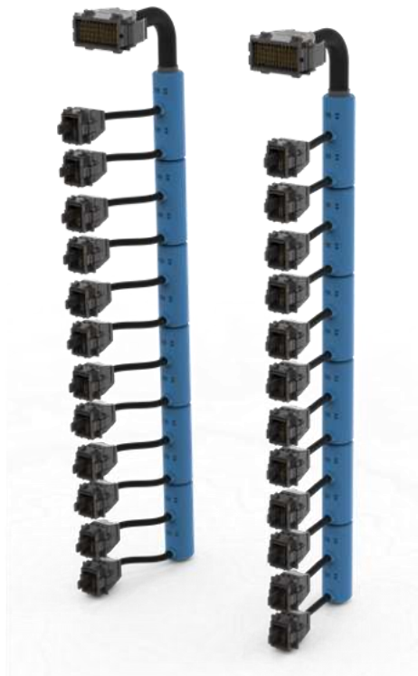
Figure 51 :Open19 12RU Data Cable 2
