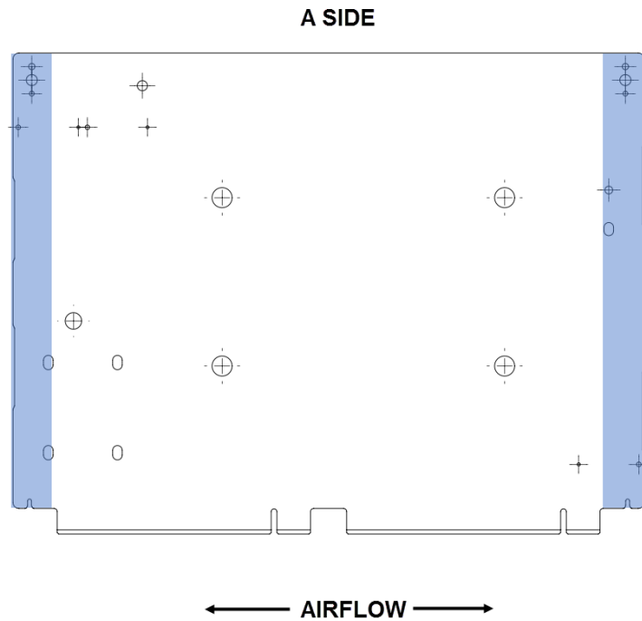
Figure 6-2 Ambient Temperature Sensor Placement Location (Highlighted Areas in Blue)
