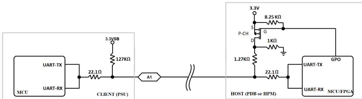
Figure 12-17 Physical layer and connections for point-to-point communication between Host and Client
