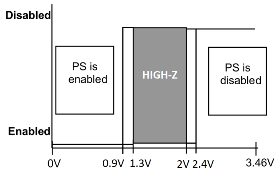
Figure 9-3 Three-state PSN# Required signal characteristics.
