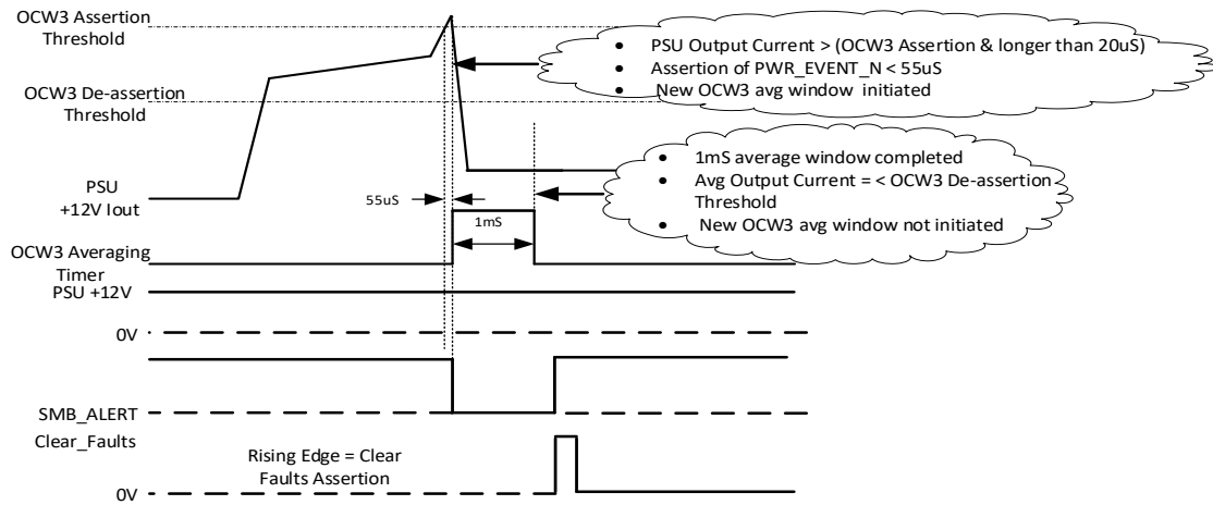
Figure 8-17 OCV3 Timing (Default Setting)
