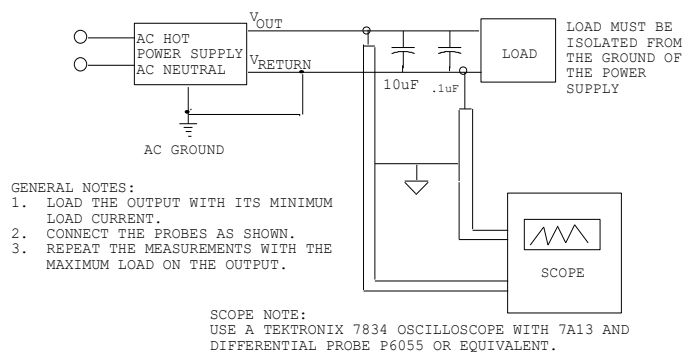
Figure 7-5 Differential noise test setup
