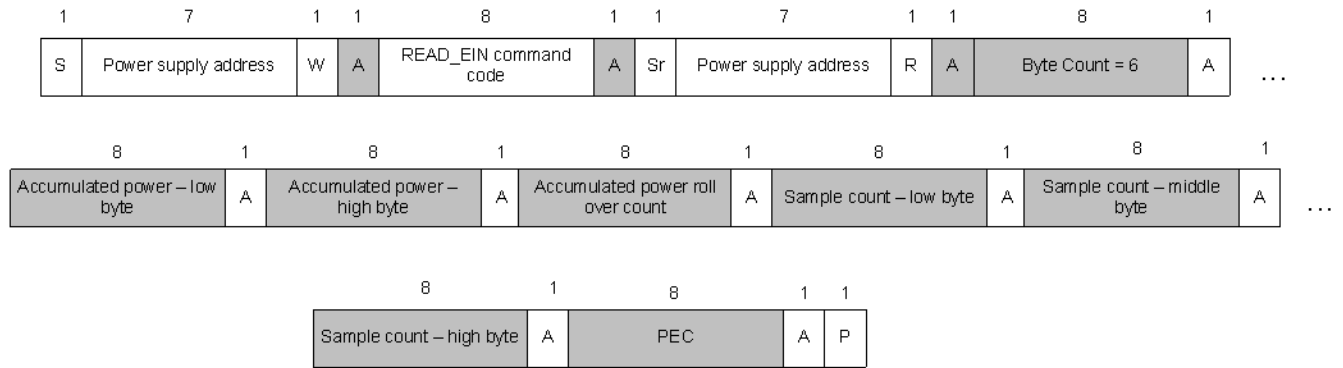
Figure 12-3 READ_EIN command format
