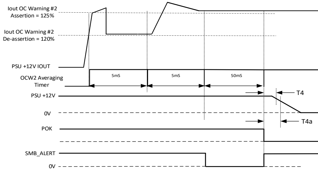
Figure 8-16 SMBAlert# assertion OCV2 Timing (Default Setting) with PWOK de-assertion
