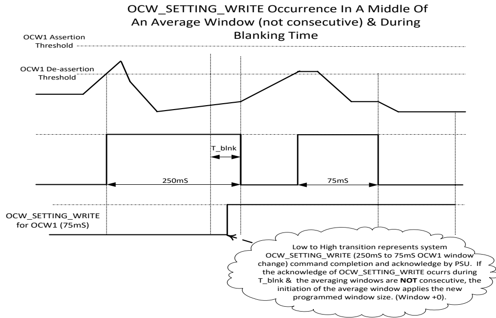
Figure 8-10 OCW1 setting
