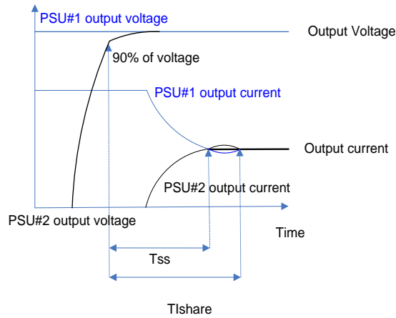
Figure 7-4 TSS and T ishare timing
