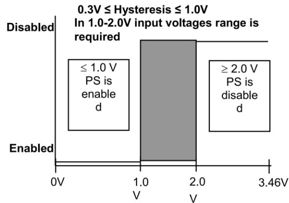
Figure 9-2 Two-state PSN# required signal characteristics.
