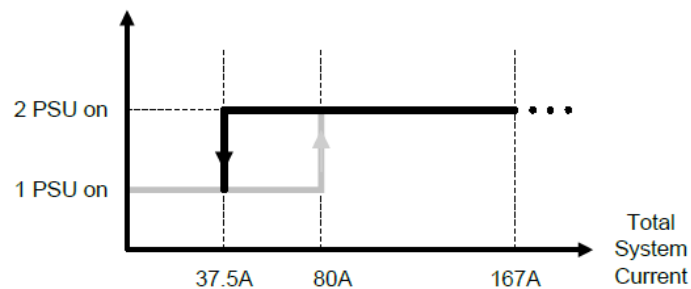
Figure 7 Hot-standby enable/disable typical current thresholds
