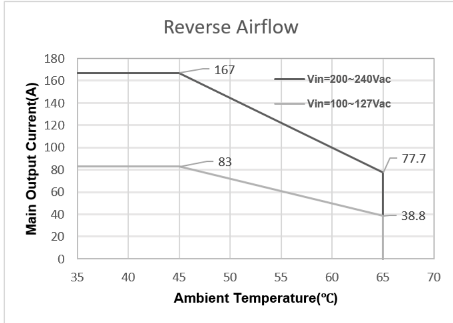
Figure 10 Iout derating with temperature (Reverse airflow)
