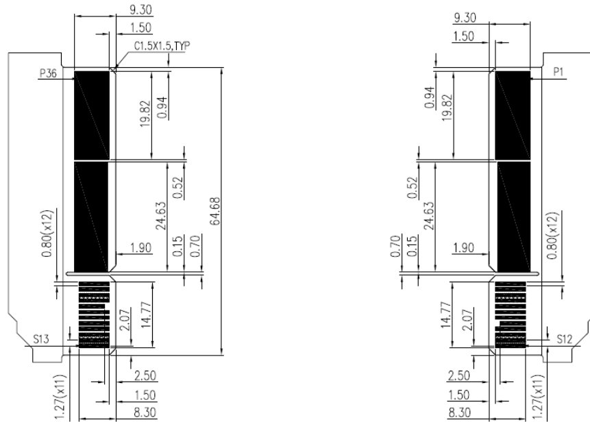
Figure 2 Detail Drawing
