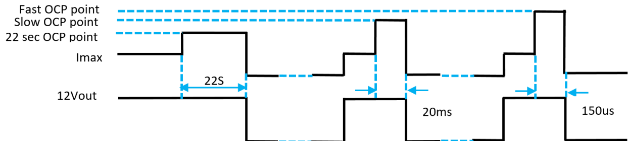
Figure 4 12V OCP latch off
