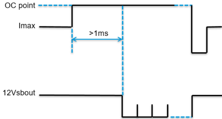
Figure 5 12Vsb OCP hiccup
