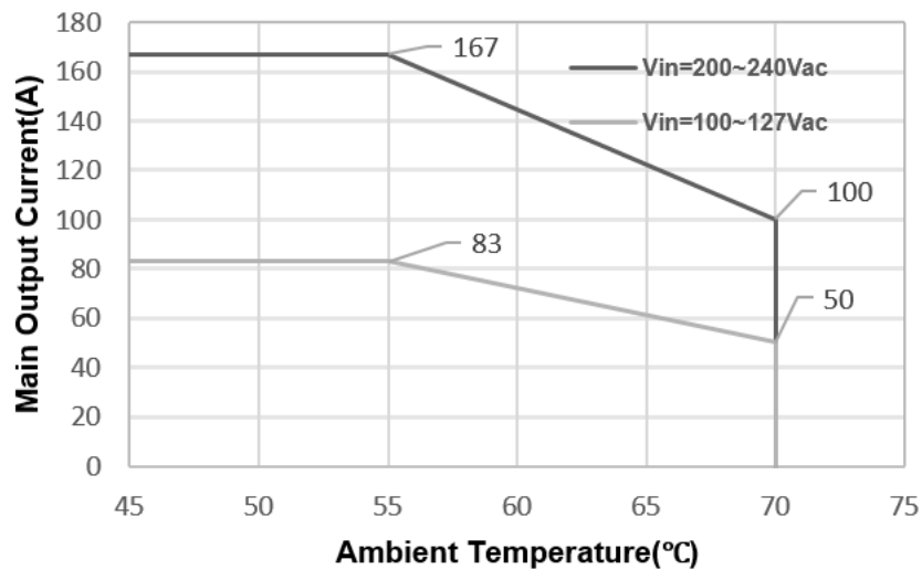
Figure 9 lout derating with temperature (Normal airflow)
