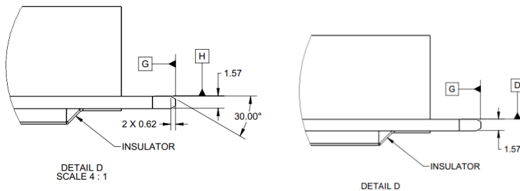
Figure 33: LFF Keep Out Zone – Side View – Detail D
