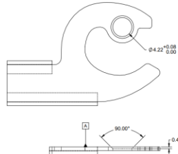
LATCH'S LEVER HOLE &amp; CHAMFER
