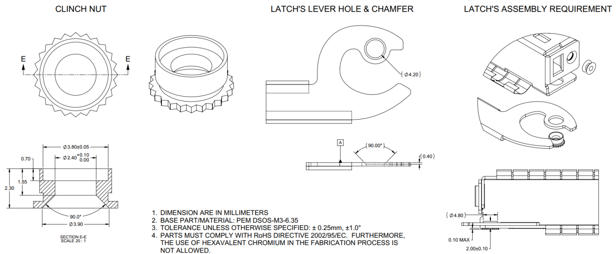
Figure 23: Clinch Nut Option B
