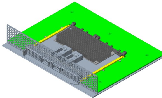
NIC Installed in Baseboard with Straddle Mount
