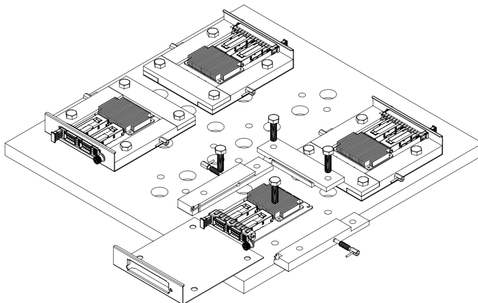
Figure 144: SFF Shock and Vibe Fixture
