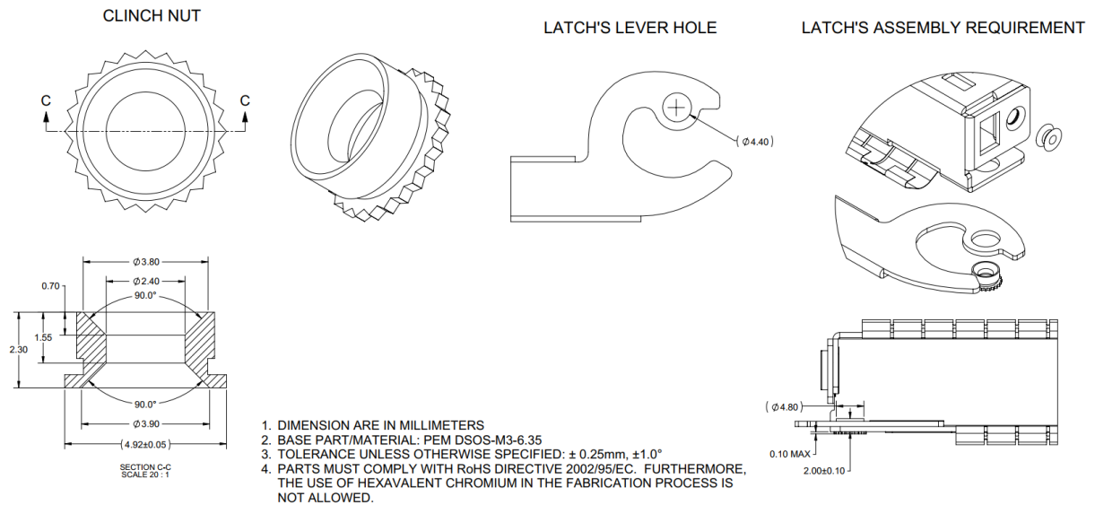
Figure 22: Clinch Nut Option A
