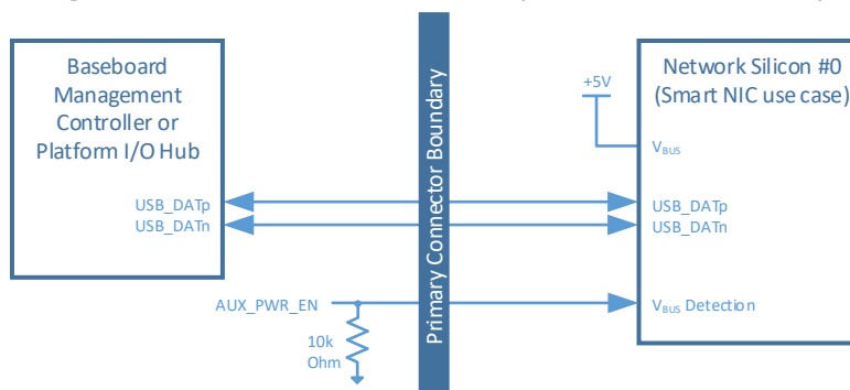
Figure 90: USB 2.0 Connection Example – Basic Connectivity
