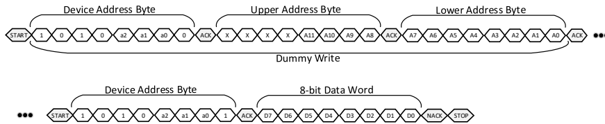
Figure 110: FRU EEPROM Reads with Double Byte Addressing
