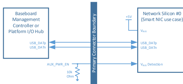
Figure 89: USB 2.0 Connection Example – Basic Connectivity
