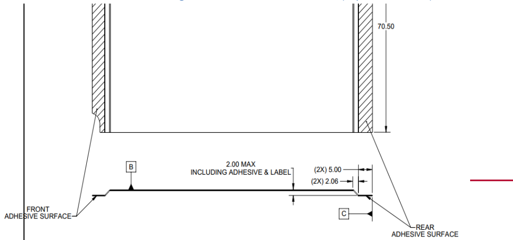
Figure 35: SFF Bottom Side Insulator (Top and Side View)
