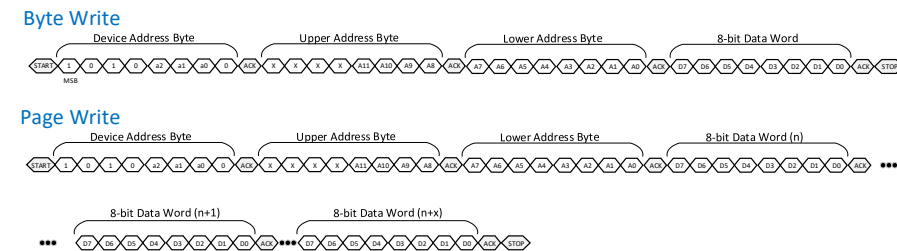
Figure 107: FRU EEPROM Writes with Double Byte Addressing
