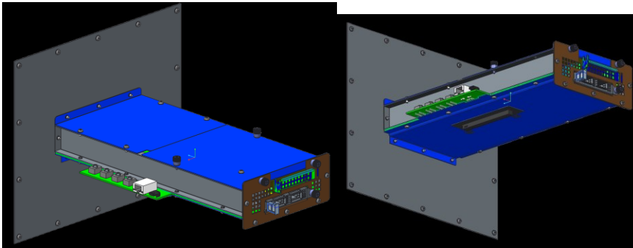
Figure 128 Figure 124 : SFF Thermal Test Fixture Preliminary Design
