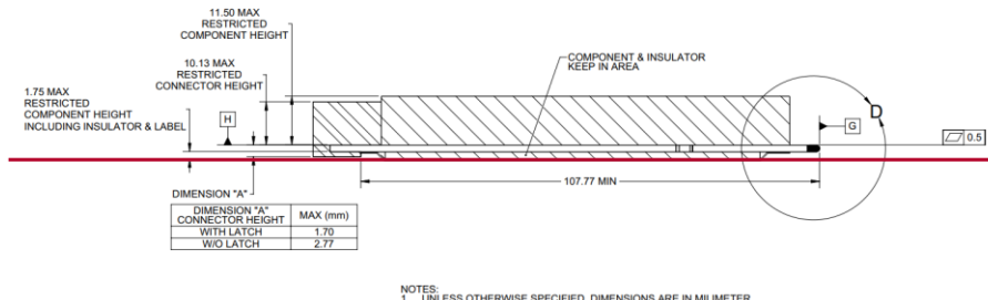
Figure 27: SFF Keep Out Zone – Side View
