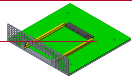
Right Angle vs Straddle Mount Chassis Configuration
