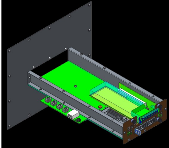
Figure 129125 : SFF Thermal Test Fixture Preliminary Design – Cover Removed
