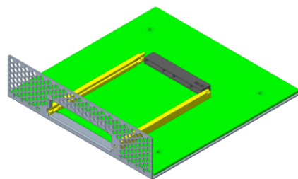
SFF with Pull Tab
