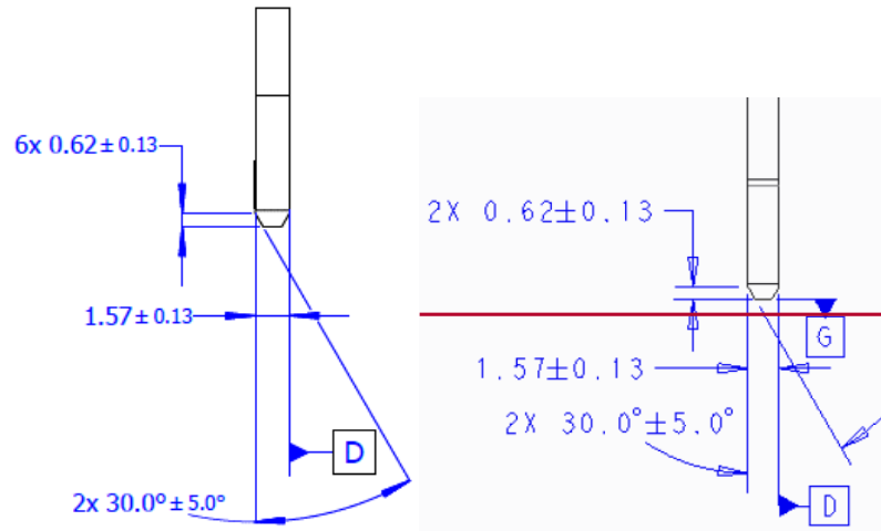
Figure 67: SFF Primary Connector Card Profile Dimensions
