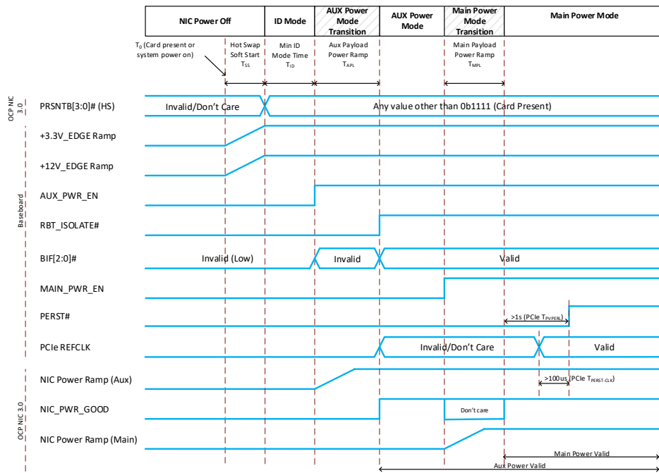
Figure 105: Power-Up Sequencing
