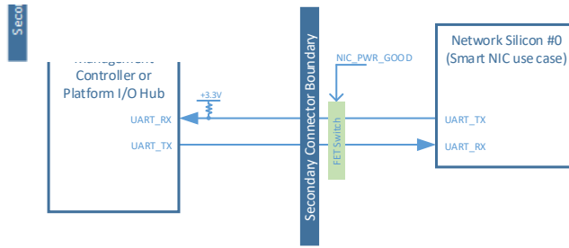
Figure 91: UART Connection Example
