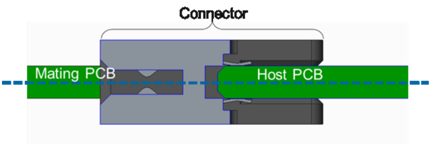
Figure 77: 0 mm Offset (Coplanar) for 0.062" Thick Baseboards
