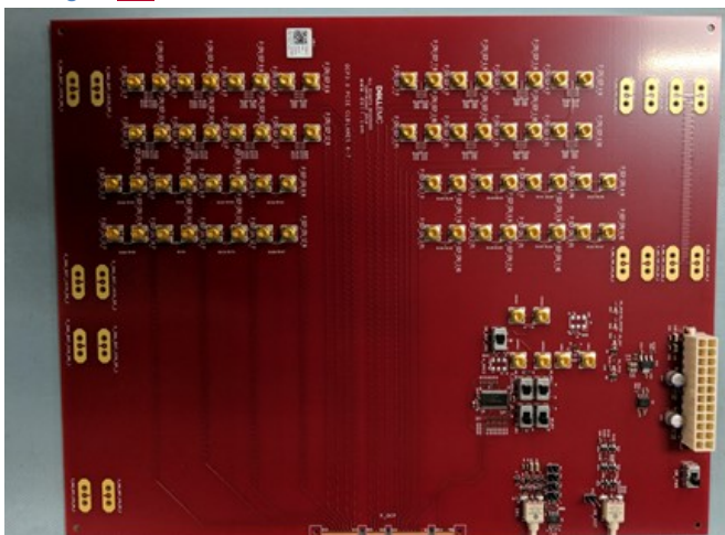
Figure 113409 : PCIe Base Board Test Fixture for OCP NIC 3.0 SFF
