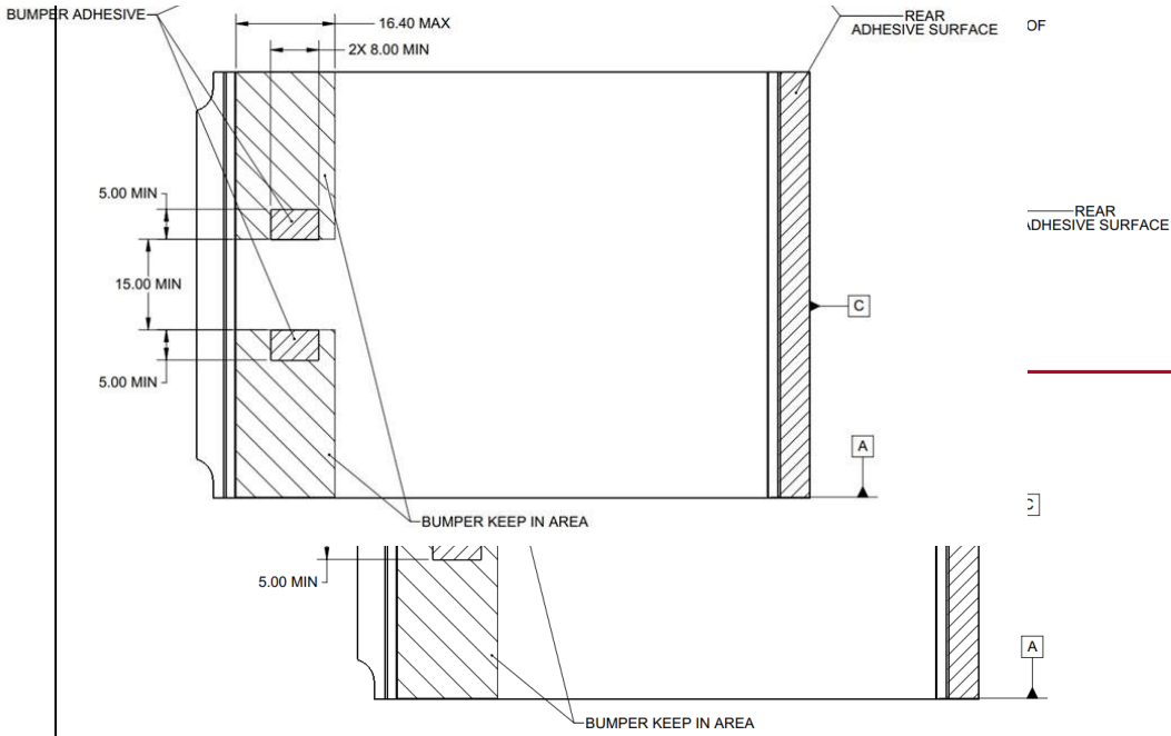
Figure 36: SFF Bottom Side Insulator (alternate) (Top and Side View)
