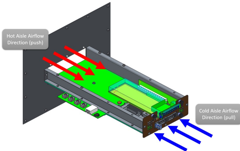
Figure 134 Figure 130: Thermal Test Fixture Airflow Direction
