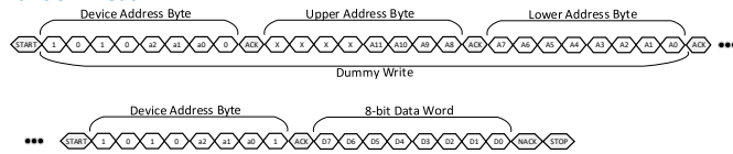
Figure 108: FRU EEPROM Reads with Double Byte Addressing
