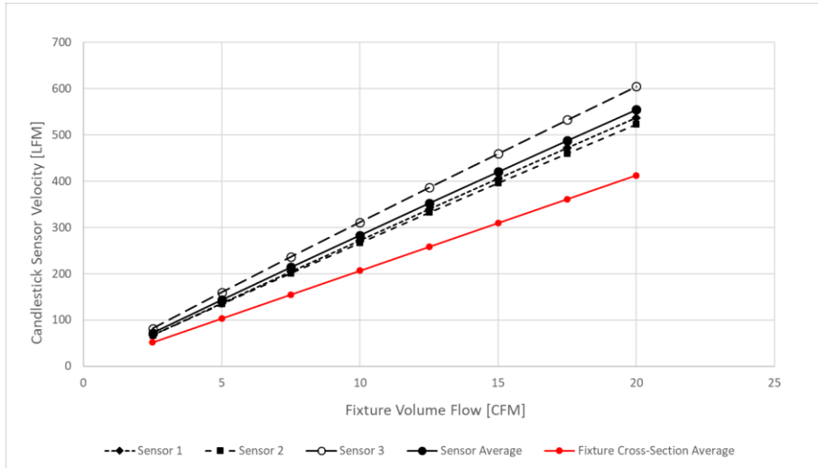
Figure 135131 136131 : SFF Fixture, Hot Aisle Flow - Candlestick Air Velocity vs. Volume Flow
