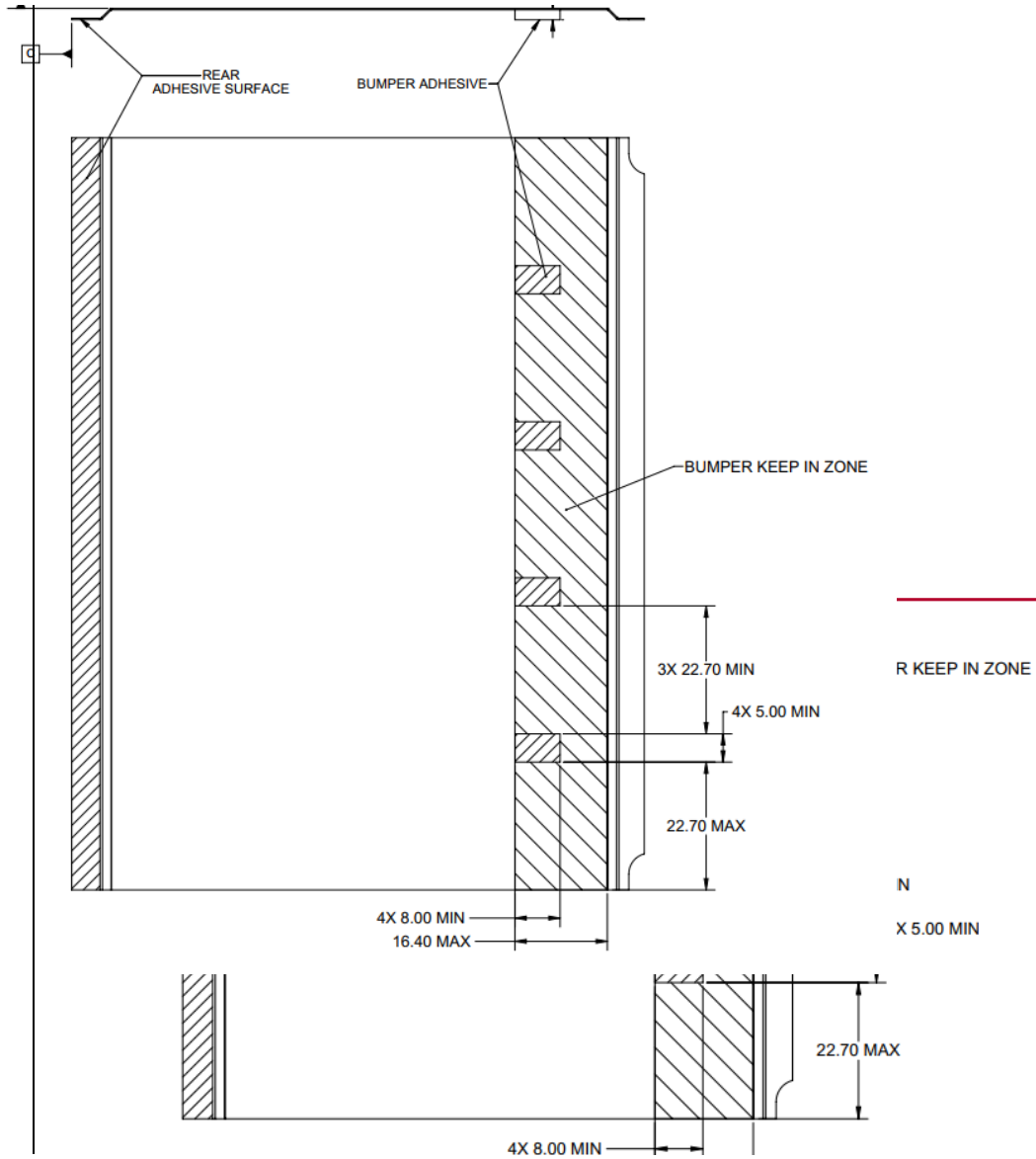
Figure 39: LFF Bottom Side Insulator (alternate) (Top and Side View)
