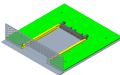
SFF with Ejector Latch
