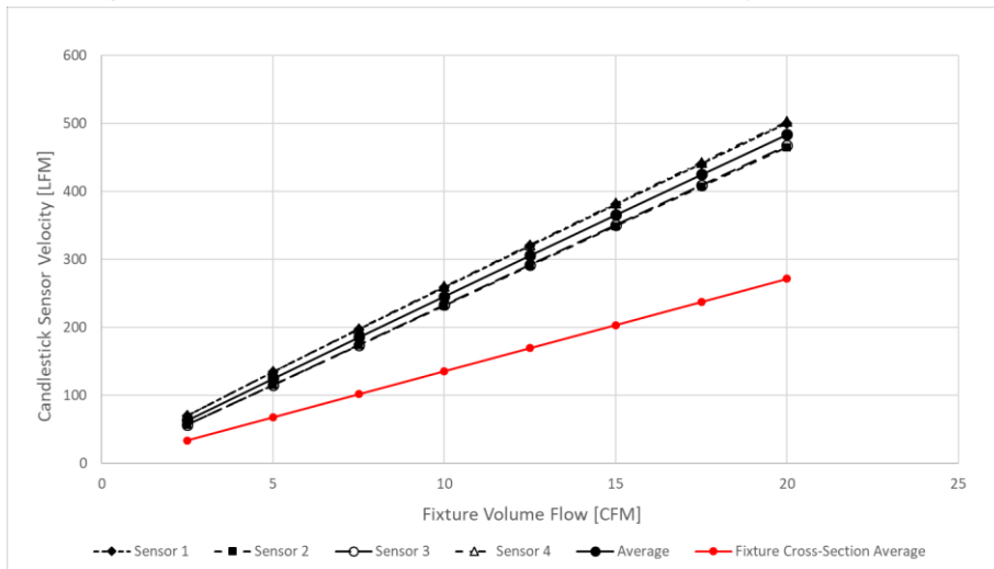
Figure 136132 136132 : LFF Fixture, Hot Aisle Flow - Candlestick Air Velocity vs. Volume Flow
