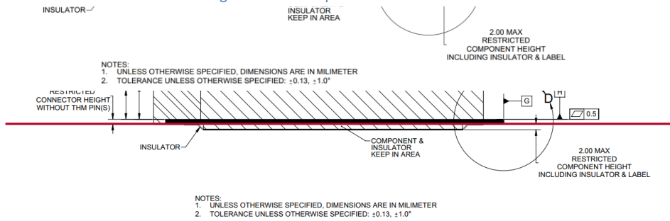
Figure 32: LFF Keep Out Zone – Side View
