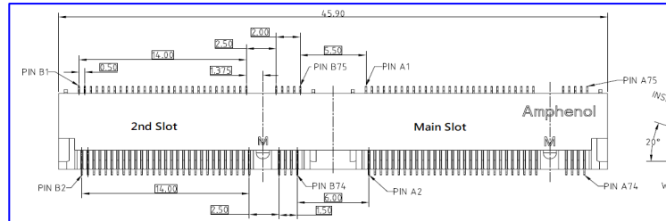
Figure 7: Dual M.2 Module and Connector Drawing
