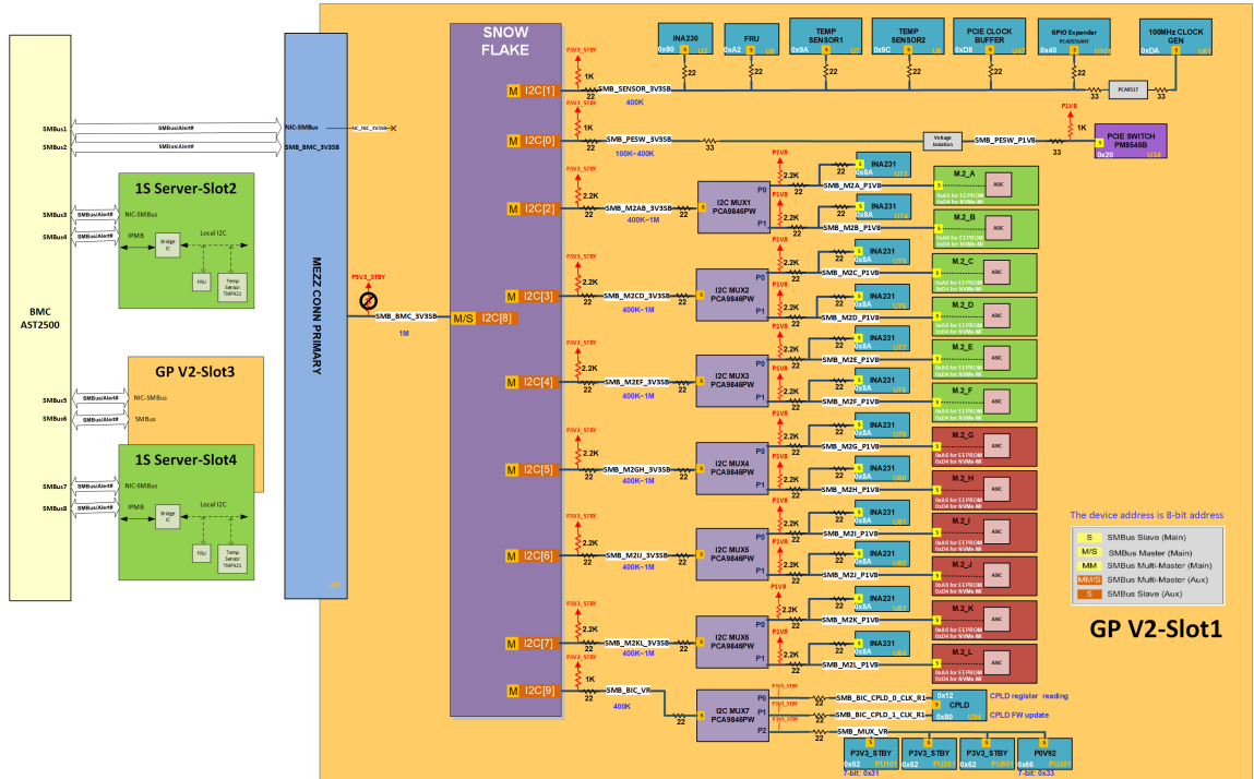
Figure 4: Typical GpV2 SMBus topology
