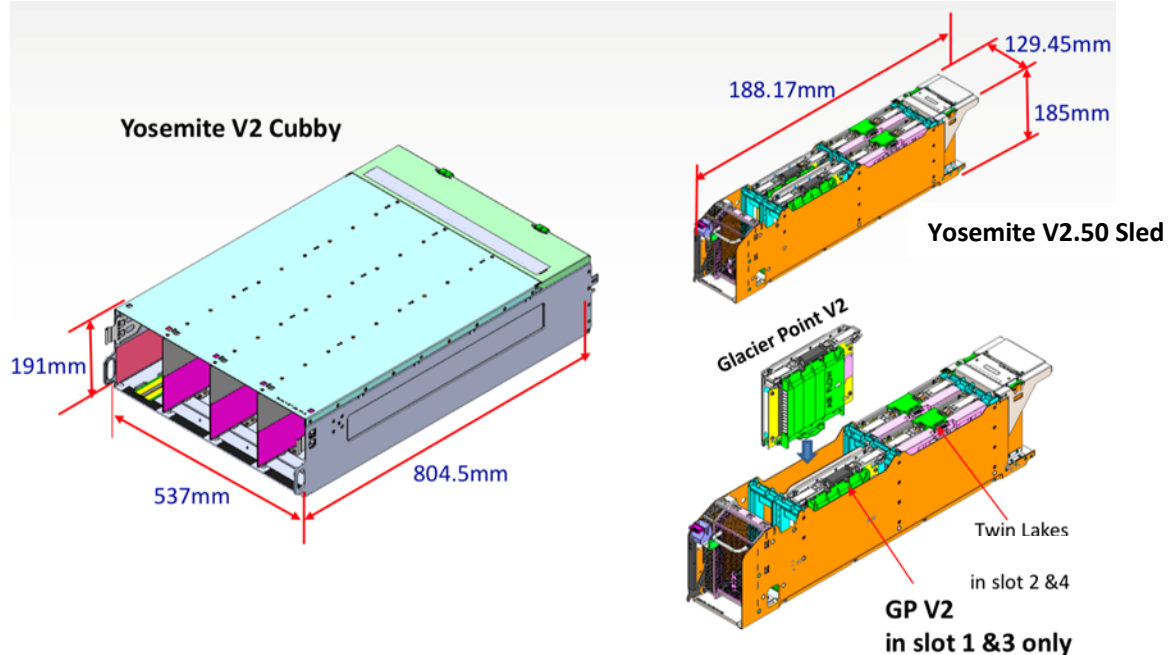
Figure 2: Yosemite V2.50 and Glacier point V2
