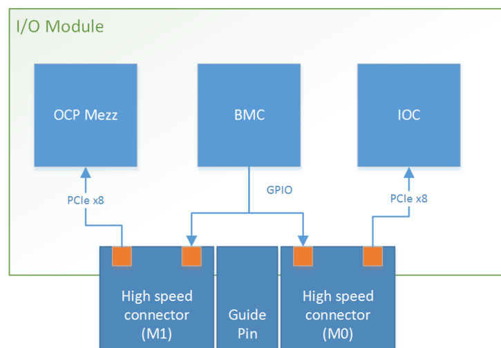
Figure 47. I/O module block diagram (NIC &amp; SAS Expansion variant)
