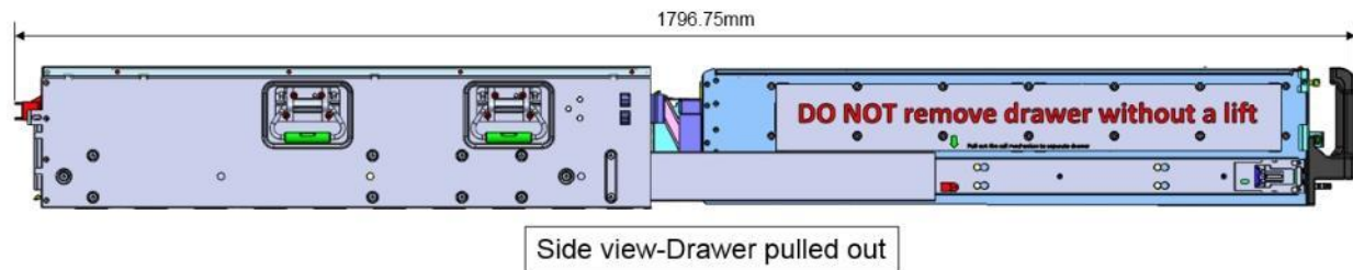
Figure 82. Dimensions with drawer pulled out
