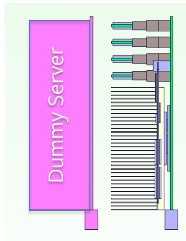
Figure 101. Dummy server installation
