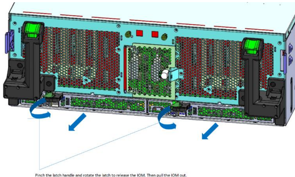
Figure 106. IOM servicing
