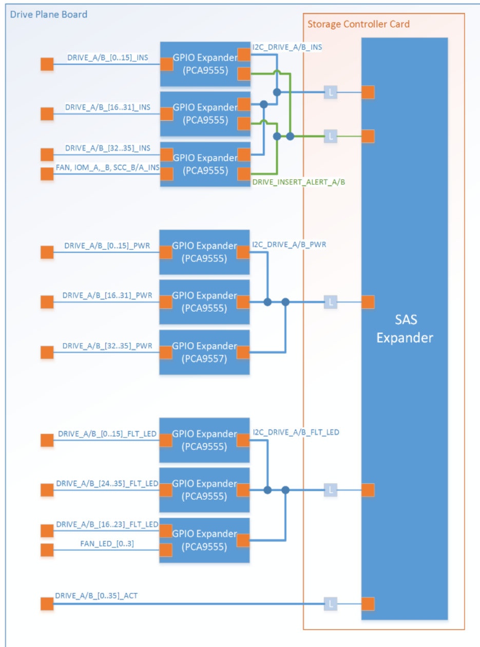
Figure 62. Drive control signal block diagram
