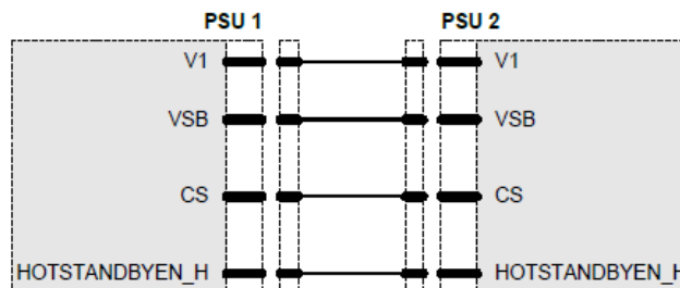
Figure 8 Recommended hot-standby configuration
