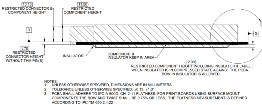
Figure 33: LFF Keep Out Zone – Side View – Detail D
