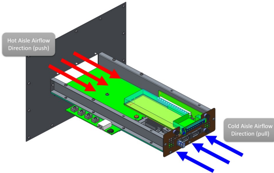
Figure 138: Thermal Test Fixture Airflow Direction
