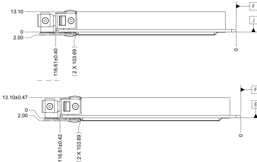
Figure 56: LFF OCP NIC 3.0 Card with Ejector CTF Dimensions (Side View)
