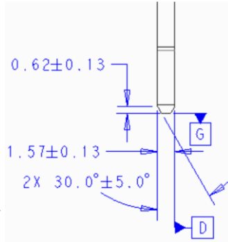
Figure 69: SFF Primary Connector Gold Finger - Detail D
