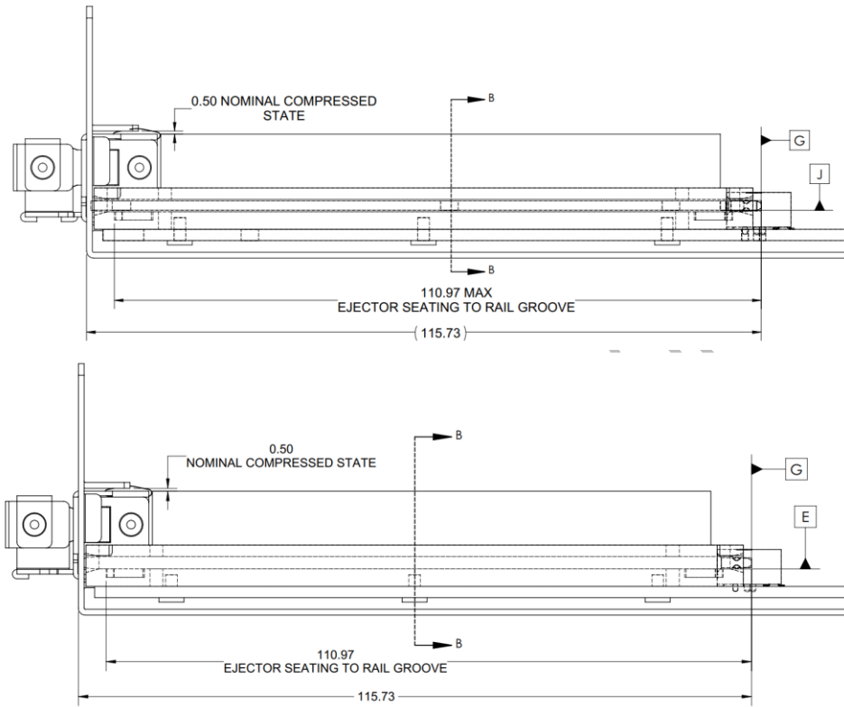
Figure 52: SFF Baseboard Chassis CTF Dimensions (Rear Rail Guide View)
