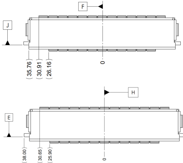
Figure 48: SFF OCP NIC 3.0 Card with Internal Lock CTF Dimensions (Side View)
