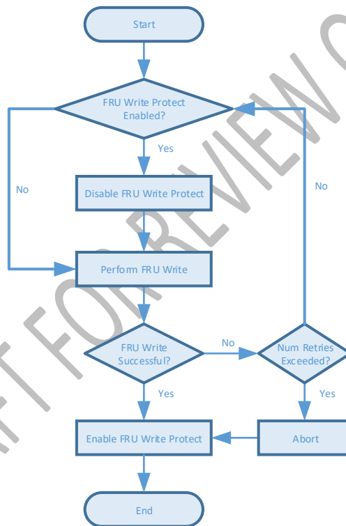
Figure 111: FRU Update Flow
