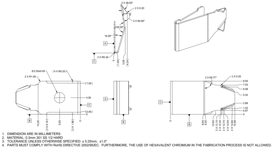
Figure 21: Ejector Lock
