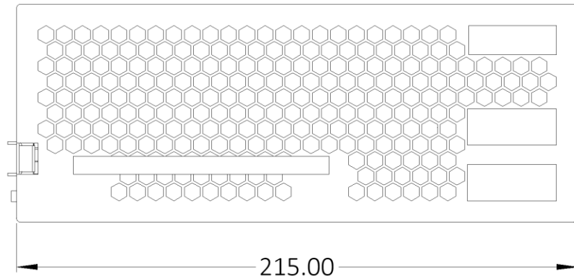
Figure 9. Half-width sled horizontal width (front view)
