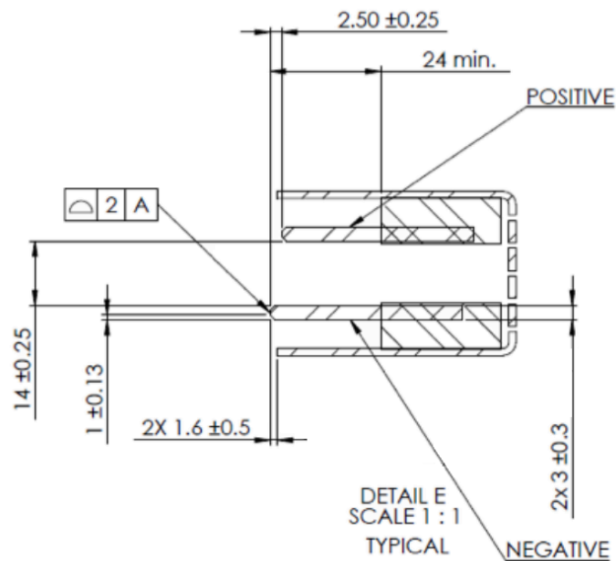
Figure 22. Bus bar pair dimensions (top view)
