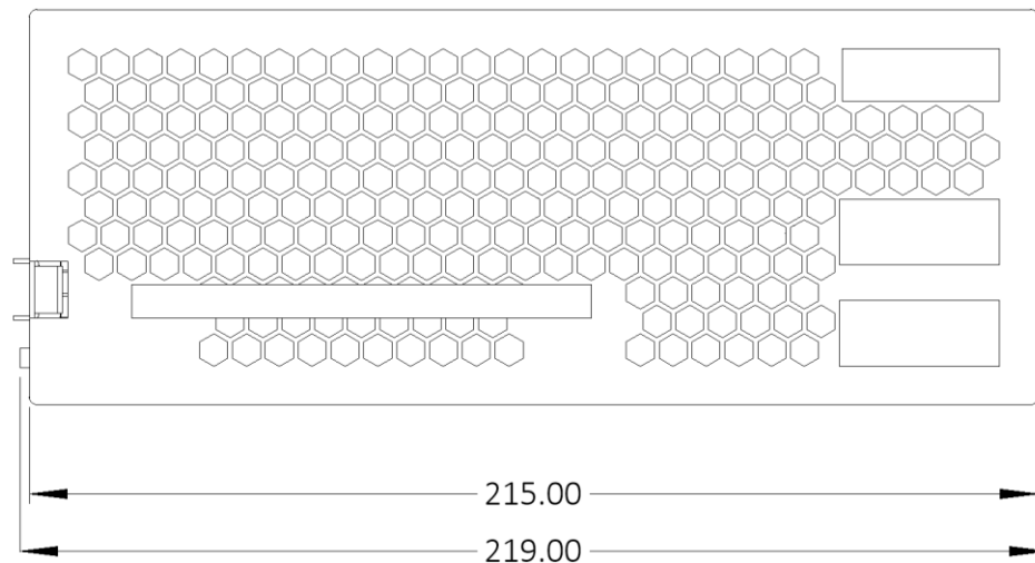
Figure 16. Sled retention pin horizontal extension (front view)
