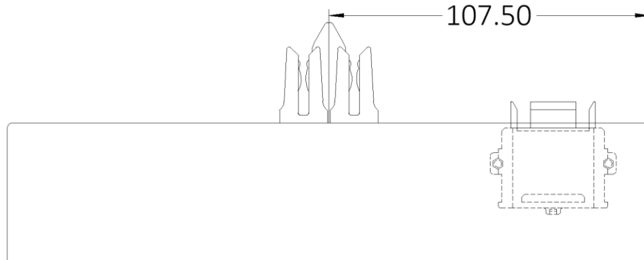
Figure 7. Sled Power connector horizontal position (top-down view)
