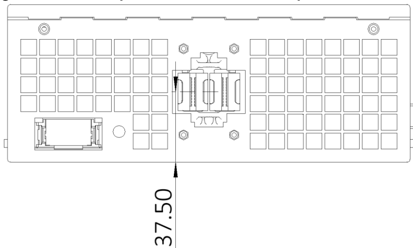
Figure 8. Sled power connector vertical position (rear view)
