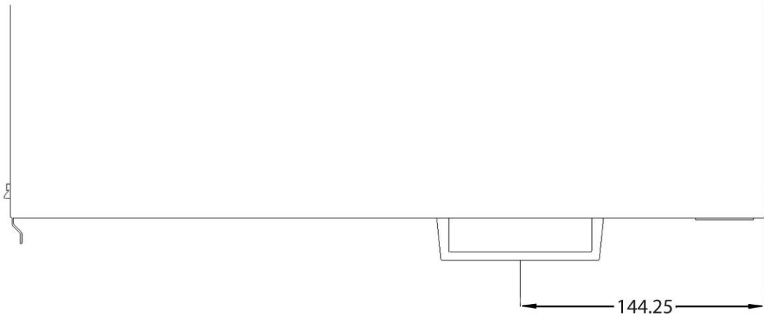
Figure 12. Full-width sled handle horizontal position (top-down view)
