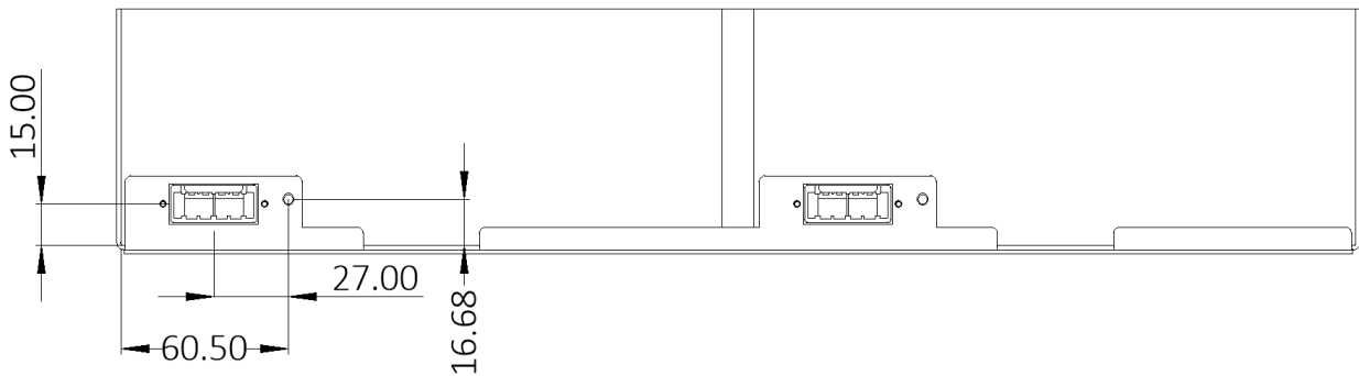
Figure 25. Shelf vertical Dimensions (rear view)
