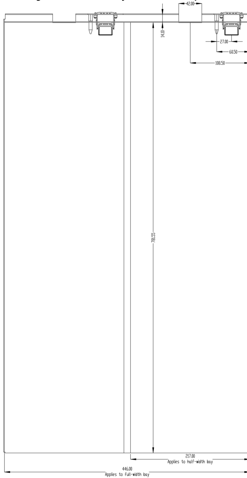
Figure 24. Shelf Bay Dimensions (top view)
