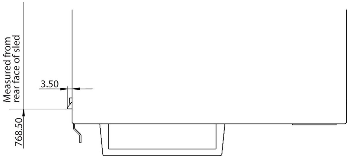
Figure 13. Sled retention latch extension (top-down view)
