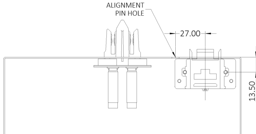
Figure 5. Sled optical connector horizontal position (top-down view)
