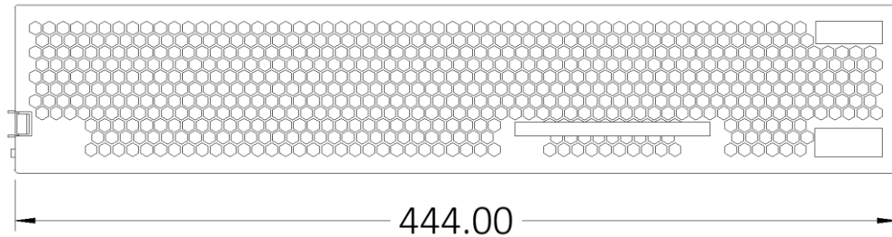
Figure 11. Full-width sled horizontal width (front view)
