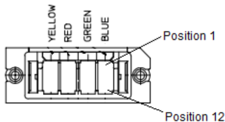
Figure 28. Sled blind-mate section assignments (rear view)
