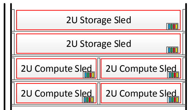
Figure 31. Sled Blind-Mate Optical Connections, Front View
