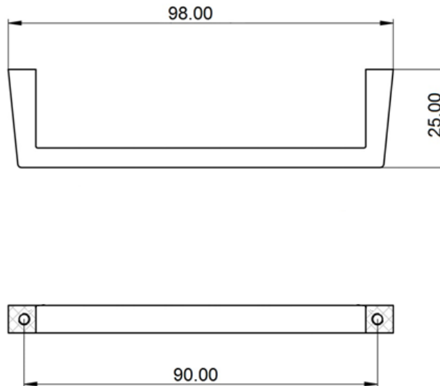
Figure 20. Sled handle dimensions
