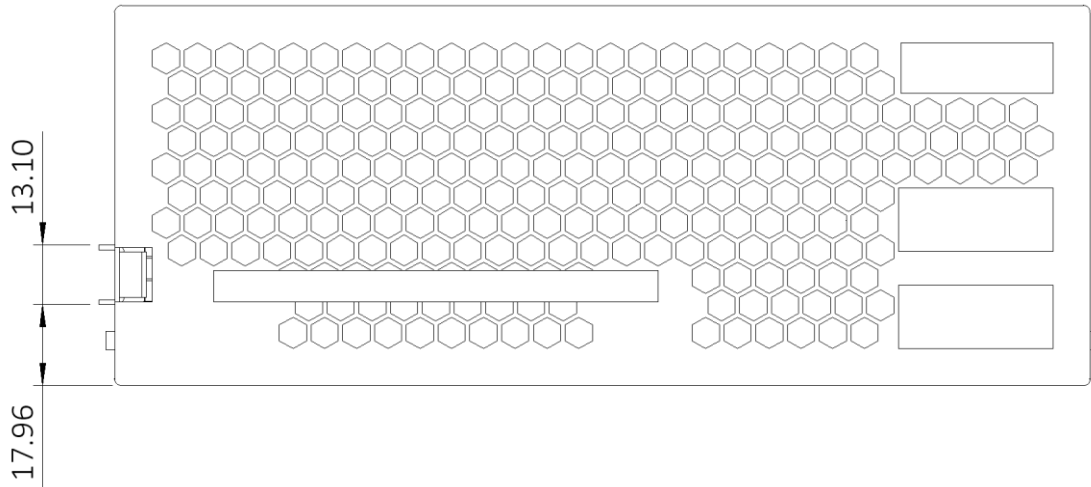
Figure 15. Sled retention latch vertical position (front view)
