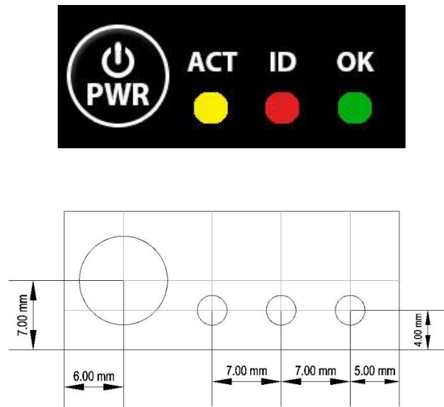
Figure 21. Sled Operator Panel Art and Dimensions
