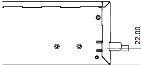
Figure 19. Sled handle vertical position (side view)
