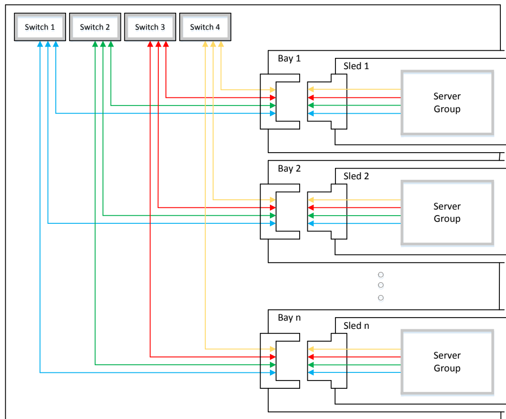
Figure 30. Network connection to sleds
