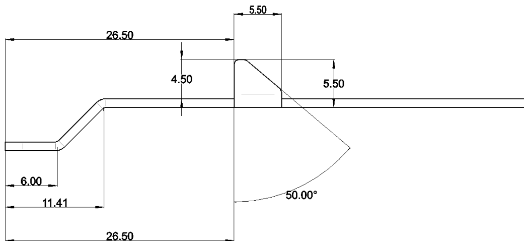
Figure 14. Example retention latch dimensions (top-down view)
