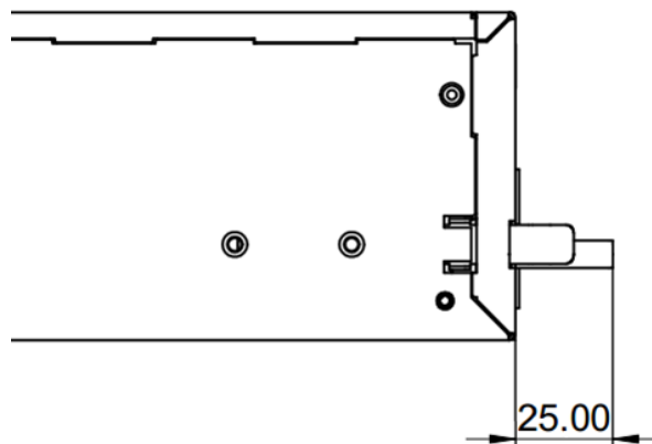
Figure 18. Sled handle horizontal extension (side view)
