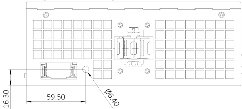
Figure 4. Sled Alignment Pin Hole (rear view)
