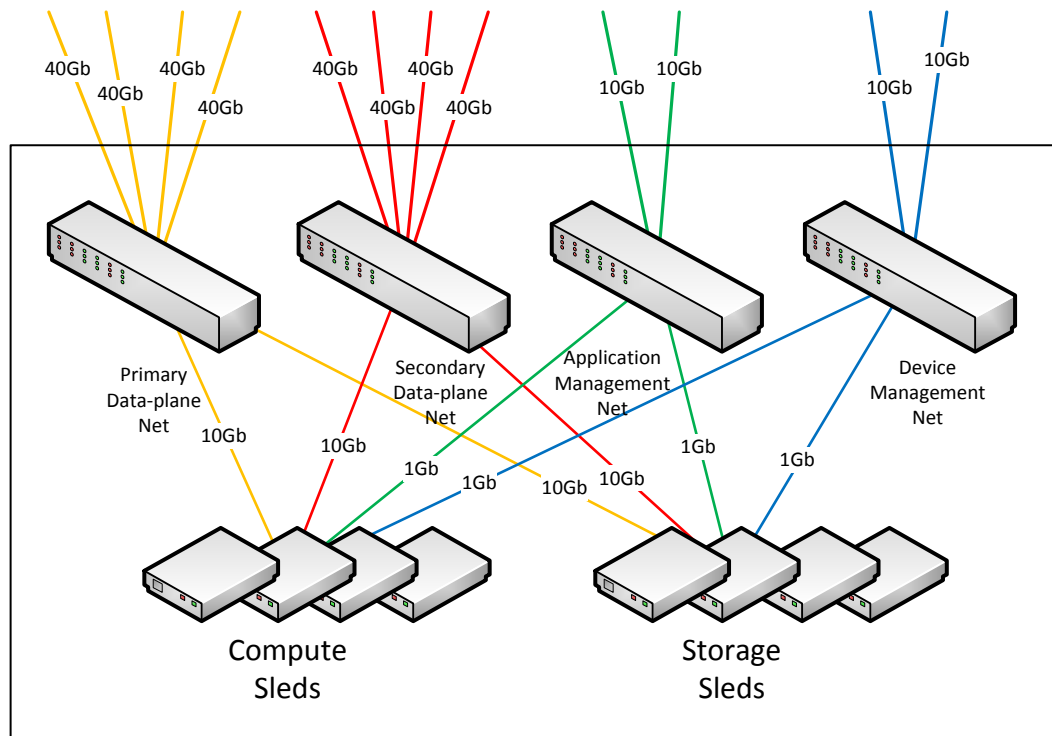
Figure 29. Example Data Plane and Management Plane Architecture
