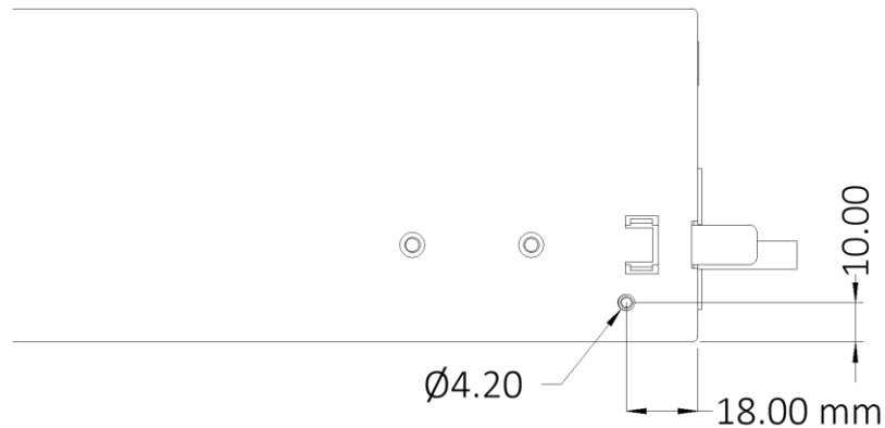
Figure 17. Sled retention pin horizontal extension (front view)
