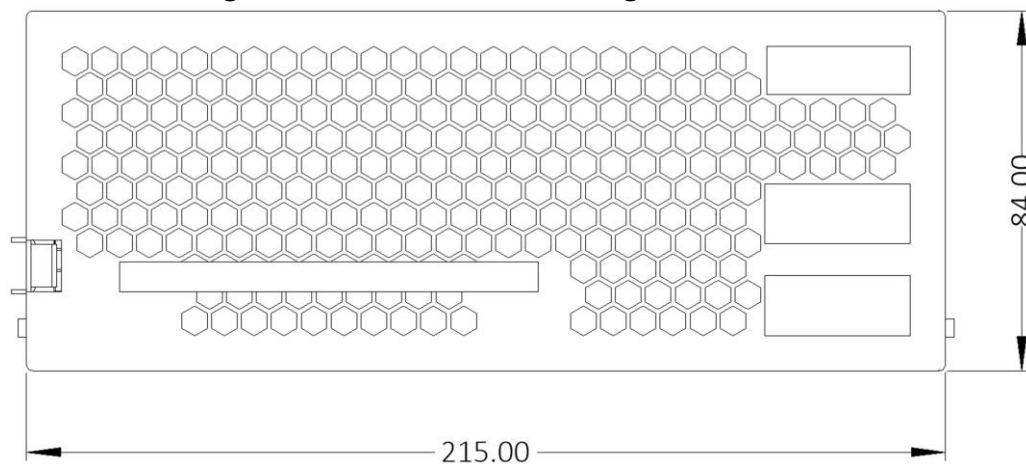
Figure 2. Sled Vertical Height (front view)
