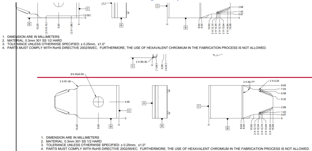
Figure 21: Ejector Lock
