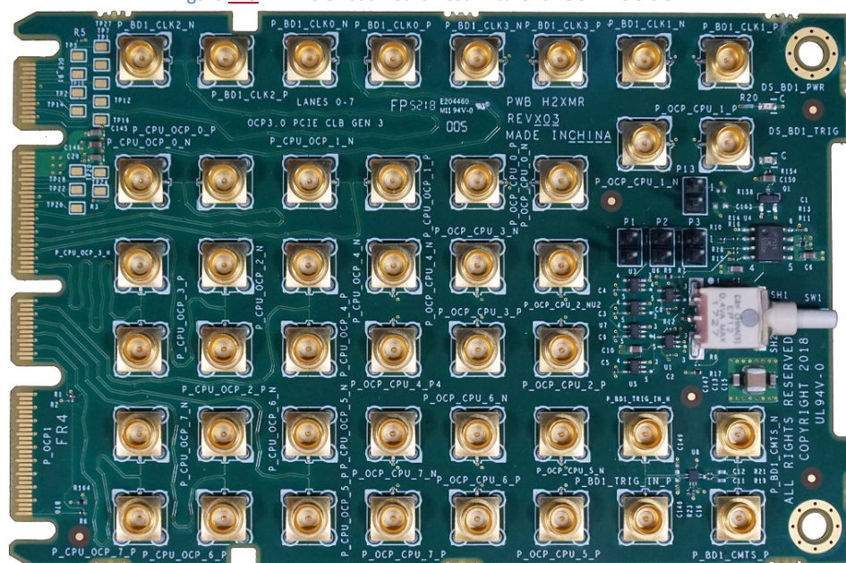
Figure 115114: PCIe Load Board Test Fixture for OCP NIC 3.0 SFF
