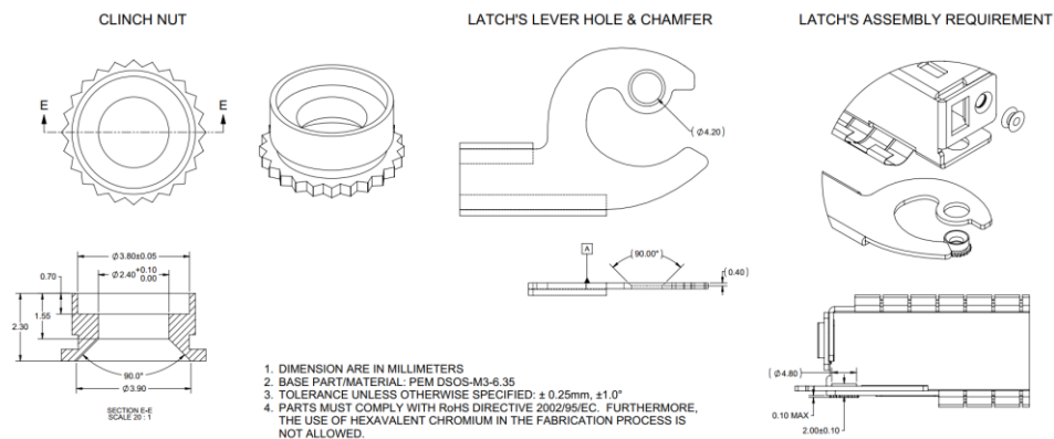
Figure 23: Clinch Nut Option B
