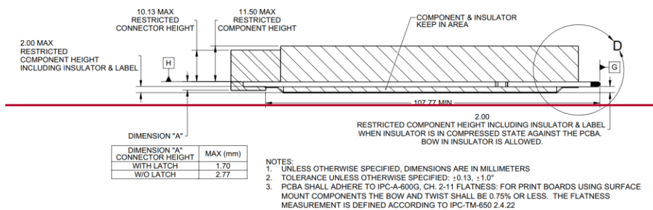
Figure 27: SFF Keep Out Zone – Side View
