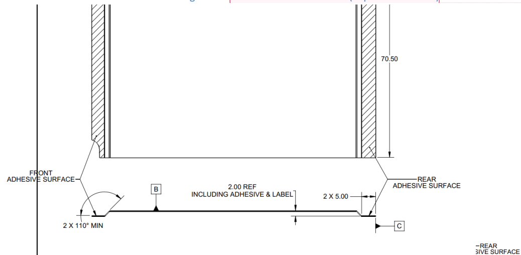
Figure 35: SFF Bottom Side Insulator (Top and Side View)
