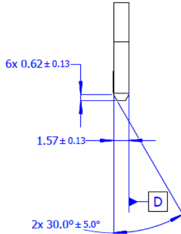
Figure 6867 : SFF Primary Connector Card Profile Dimensions
