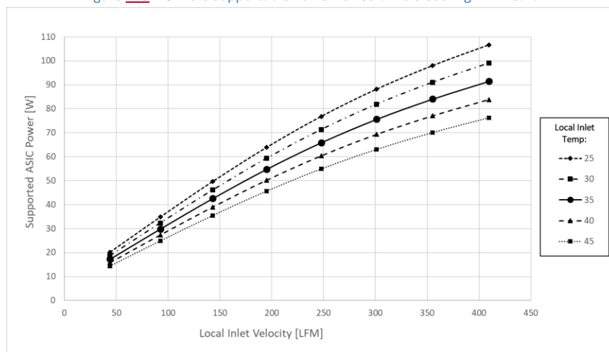
Figure 129 Figure 128 : ASIC Supportable Power for Cold Aisle Cooling – LFF Card
