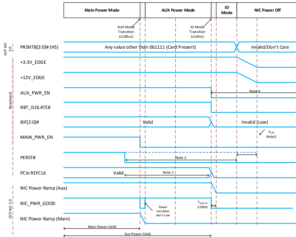
Figure 107106 107106: Power-Down Sequencing – Normal Operation
