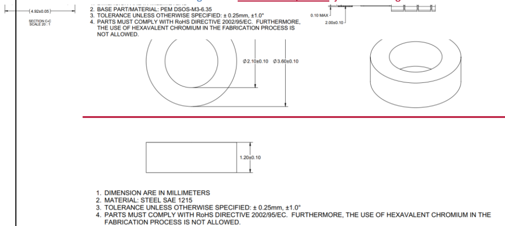
Figure 22: Clinch Nut Option A Ejector Bushing
