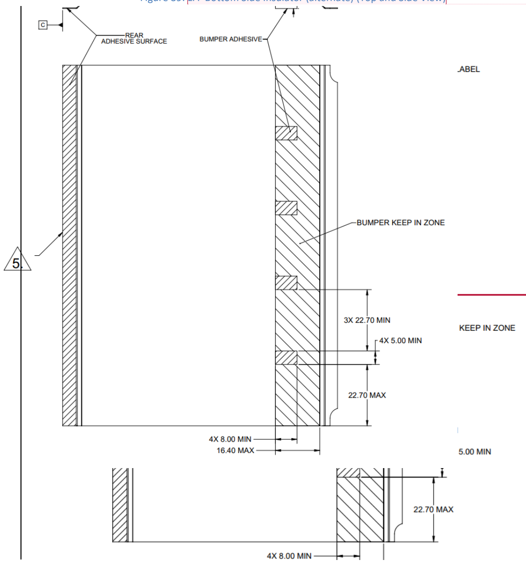
Figure 39: LFF Bottom Side Insulator (alternate) (Top and Side View)
