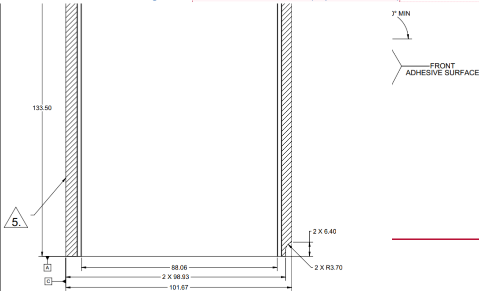
Figure 38: LFF Bottom Side Insulator (Top and Side View)
