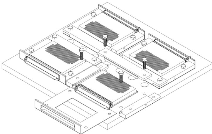
Figure 145144 : LFF Shock and Vibe Fixture
