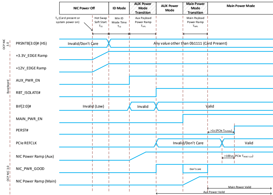
Figure 106105 106105: Power-Up Sequencing – Normal Operation
