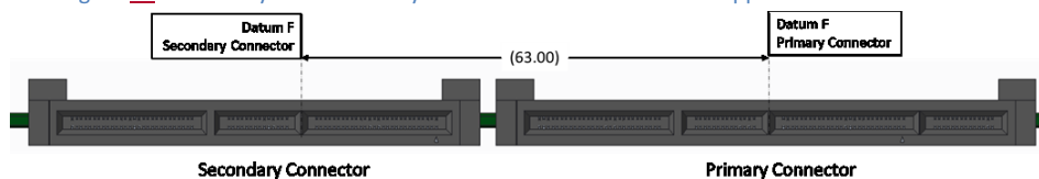
Figure 8180 : Primary and Secondary Connector Locations for LFF Support with Straddle Mount
