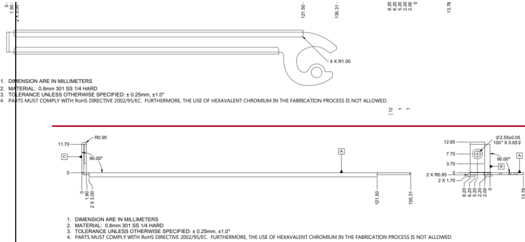
Figure 20: LFF I/O Faceplate – Ejector Lever (2D View)
