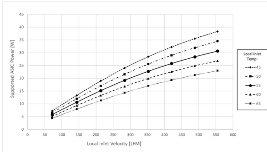
Figure 119418: ASIC Supportable Power for Hot Aisle Cooling – SFF
