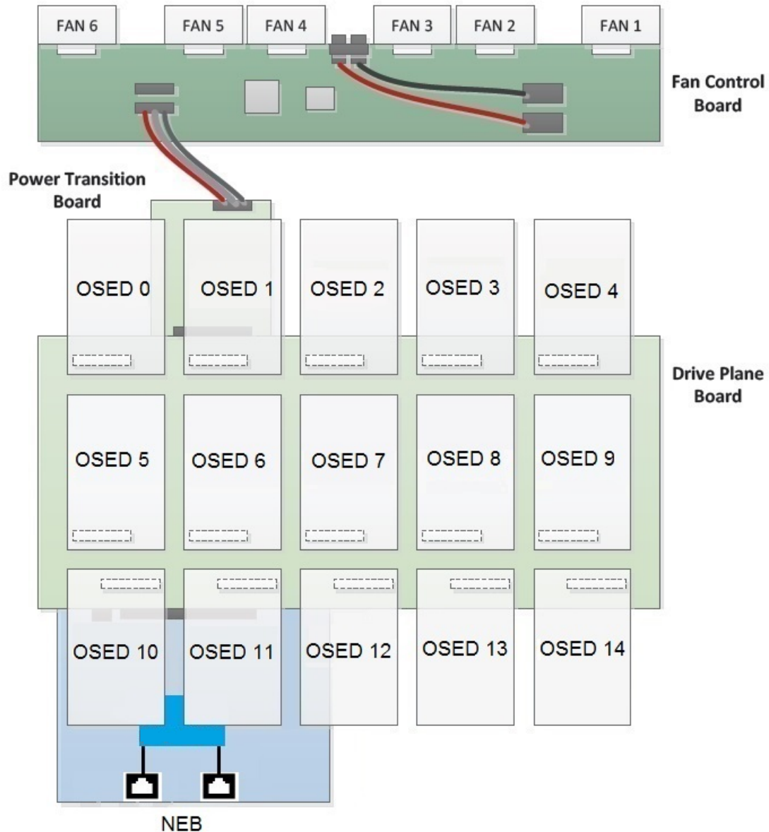
Figure 6 HDD tray diagram using OSEDs and NEBs
