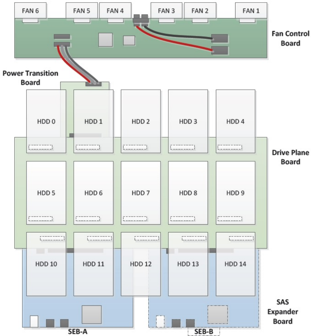
Figure 3 HDD tray diagram
