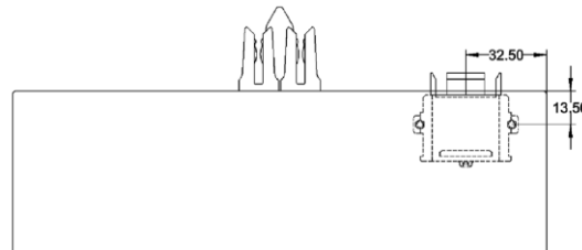
Figure 5. Sled optical connector horizontal position (top-down view)
