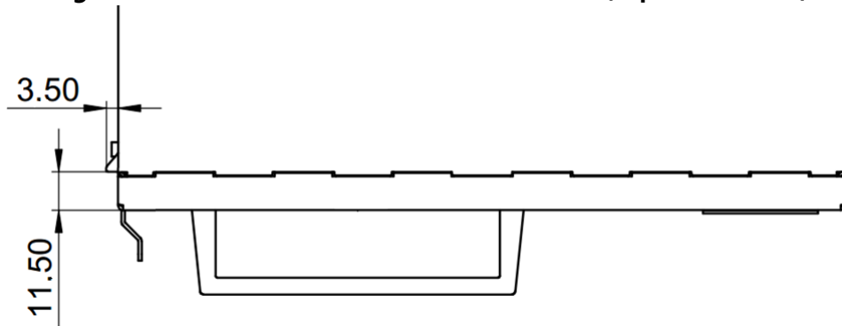
Figure 13. Sled retention latch extension (top-down view)
