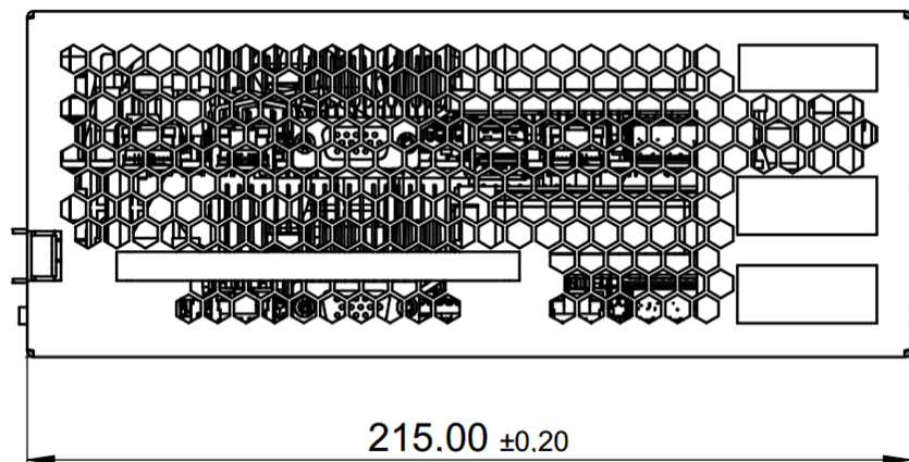
Figure 9. Half-width sled horizontal width (front view)
