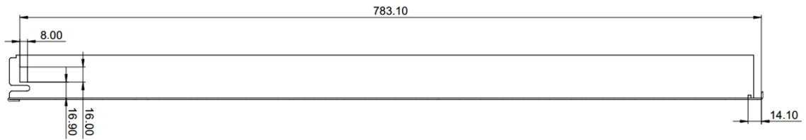
Figure 25. Shelf latch opening locations
