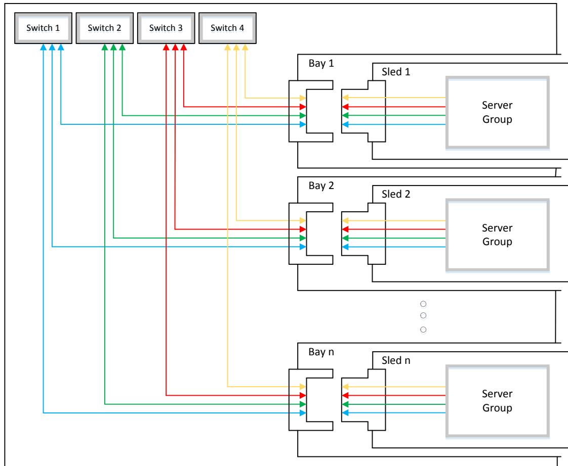
Figure 28. Network connection to sleds
