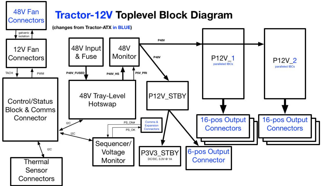
Figure 3: Tractor-12V Conceptual Block Diagram
