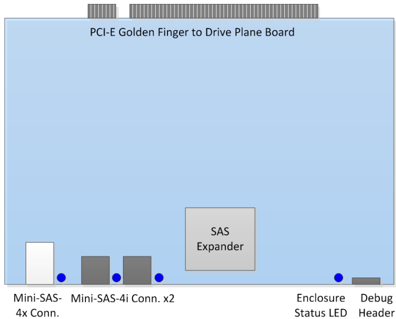
Figure 9 Open Vault SAS Expander Board Placement
