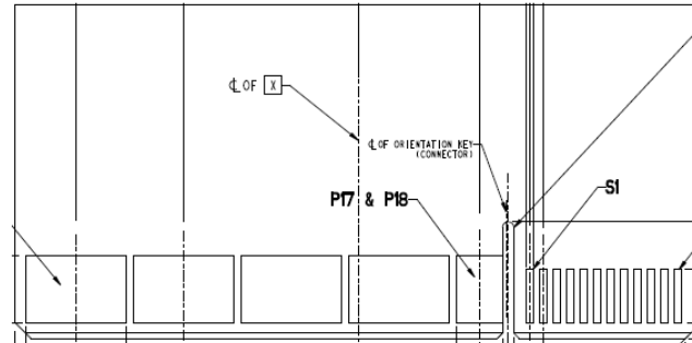
Figure 34 Golden Finger on PTB to DPB
