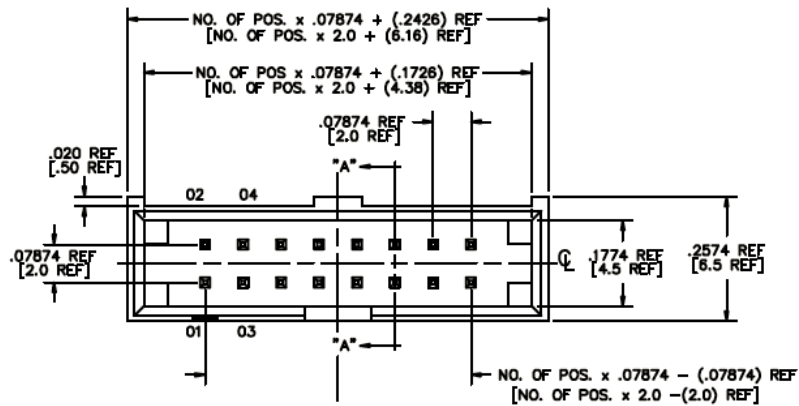
Figure 14 Debug Header
