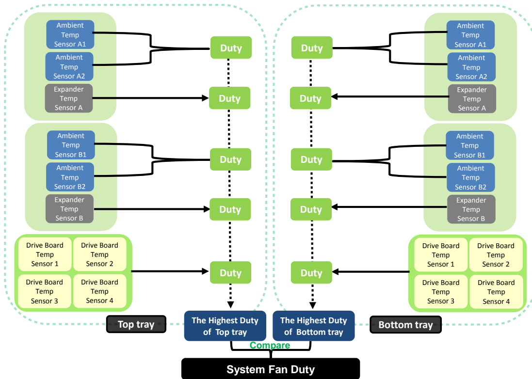
Figure 58 Open Vault System Fan Speed Control Strategy
