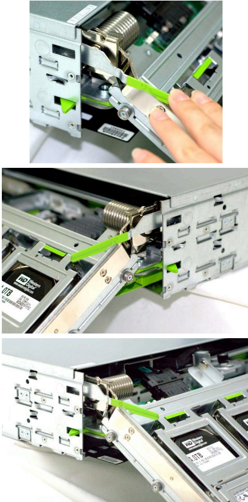
Figure 63 Front View of HDD Tray in Service
