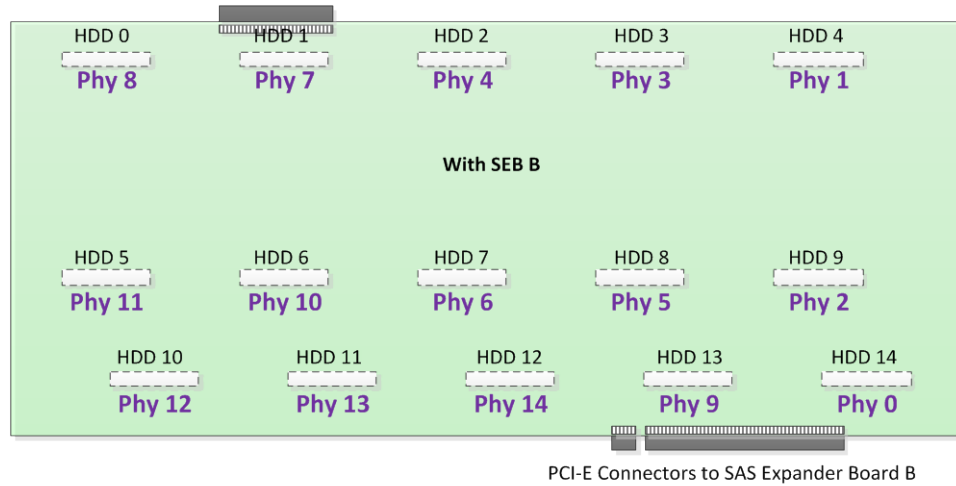
Figure 23 Open Vault DPB HDD Port Mapping on B-side
